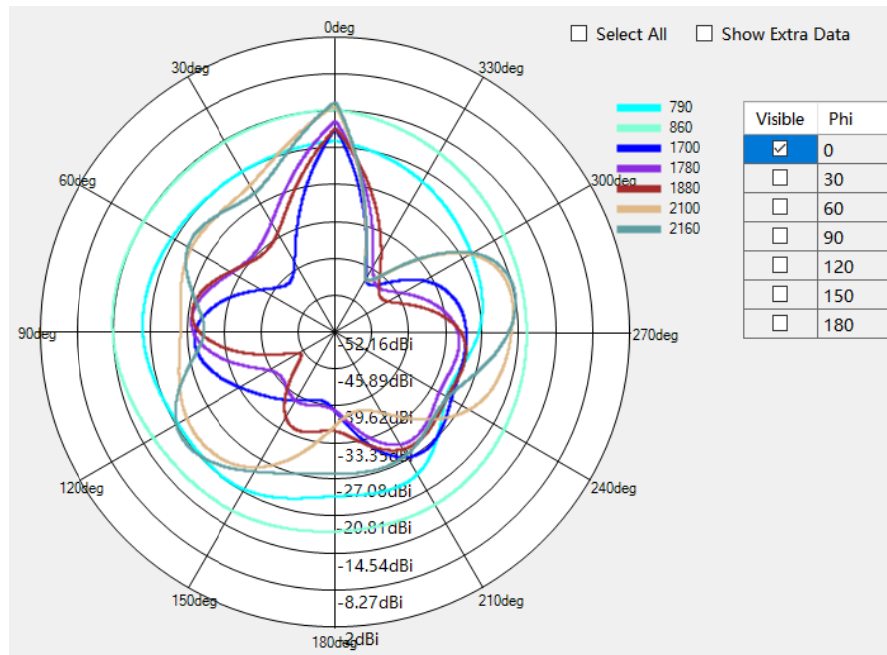
DCS1800/WCDMA B4/ LTEB3/B4/B20Phi=0deg
