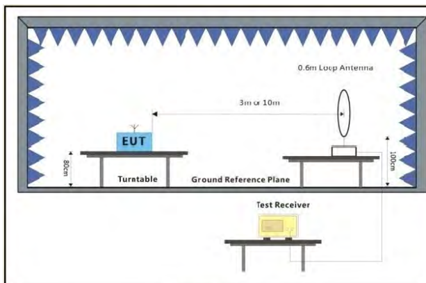
Below 30MHz
