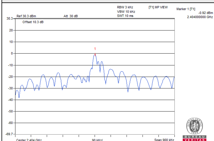
1MBaud PHY with Channel Sounding : CH 2
