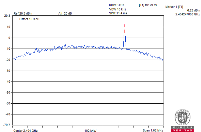
1MBaud PHY with 1Mbps : CH 1
