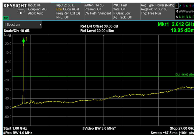
Channel: MIDDLE, Modulation: 64QAM, BW=70MHz, Range: Upper
