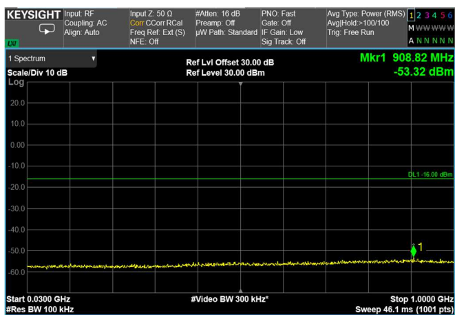
Channel: BOTTOM, Modulation: 64QAM, BW=70MHz, Range: Lower
