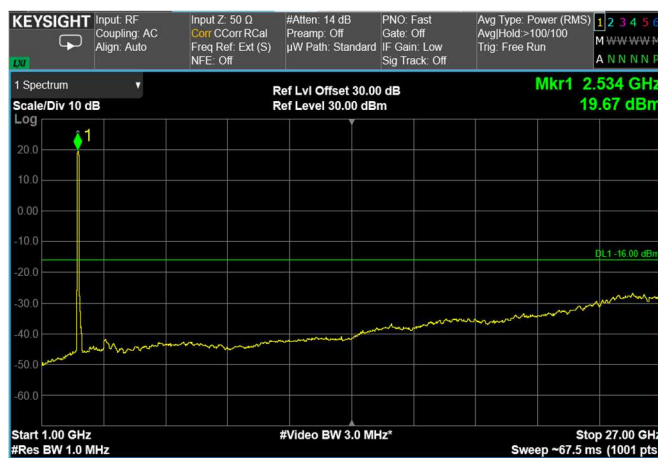
Channel: BOTTOM, Modulation: 64QAM, BW=70MHz, Range: Upper
