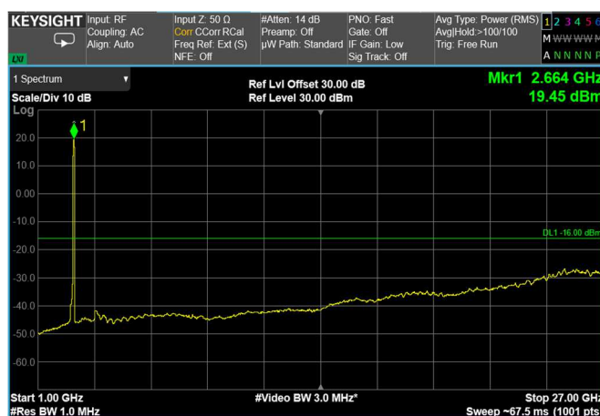
Channel: TOP, Modulation: 64QAM, BW=70MHz, Range: Upper
