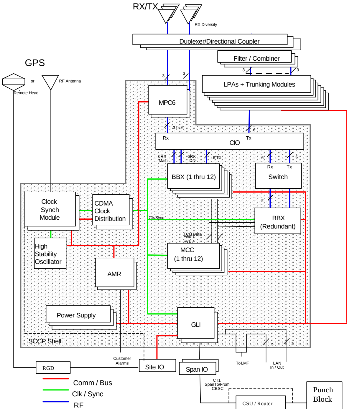
SC4812ET Functional Block Diagram
