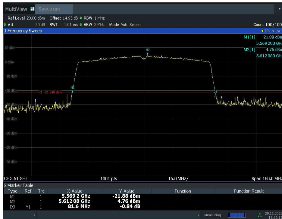
Fig.32 Occupied 26dB Bandwidth (802. 11ac-VHT80, 5610MHz)
