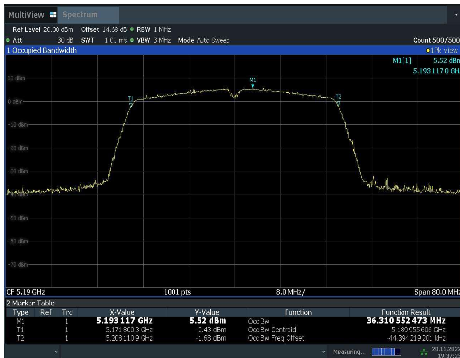
Fig.40 99% Occupied bandwidth (802.11n-HT40, 5190MHz)
