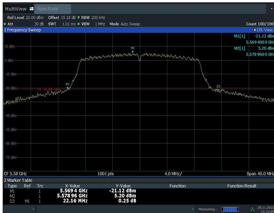
Fig.18 Occupied 26dB Bandwidth (802. 11ac-VHT20, 5580MHz)
