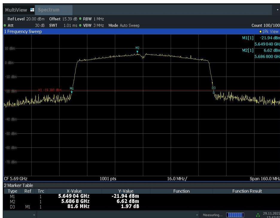
Fig.33 Occupied 26dB Bandwidth (802. 11ac-VHT80, 5690MHz)
