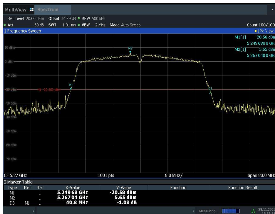
Fig.23 Occupied 26dB Bandwidth (802.11n-HT40, 5270MHz)
