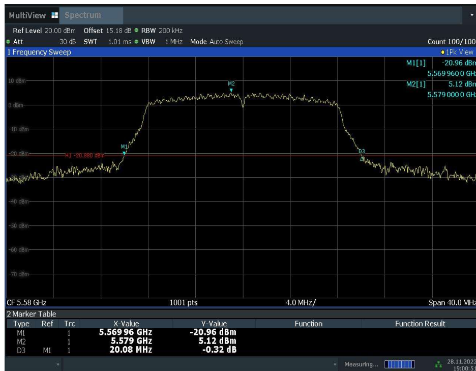
Fig.8 Occupied 26dB Bandwidth (802.11a, 5580MHz)
