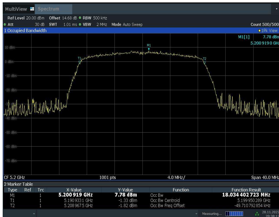
Fig.38 99% Occupied bandwidth (802.11ac-VHT20, 5200MHz)
