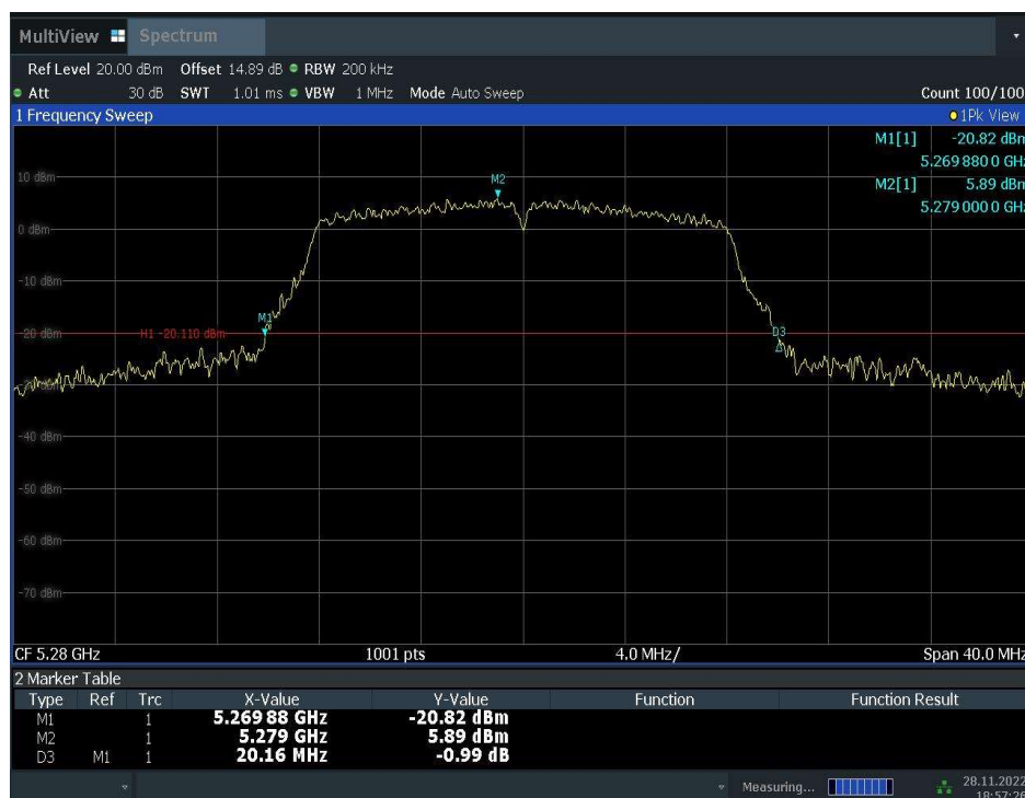
Fig.5 Occupied 26dB Bandwidth (802.11a, 5280MHz)
