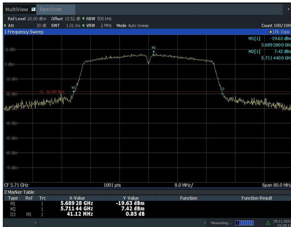
Fig.28 Occupied 26dB Bandwidth (802. 11n-HT40, 5710MHz)
