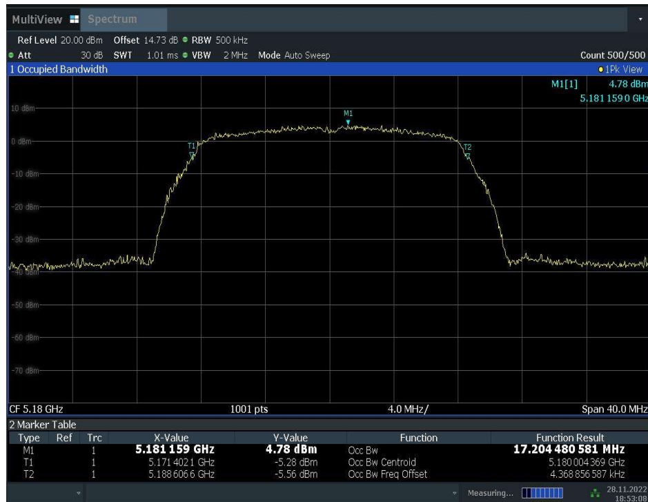
Fig.34 99% Occupied bandwidth (802.11a, 5180MHz)
