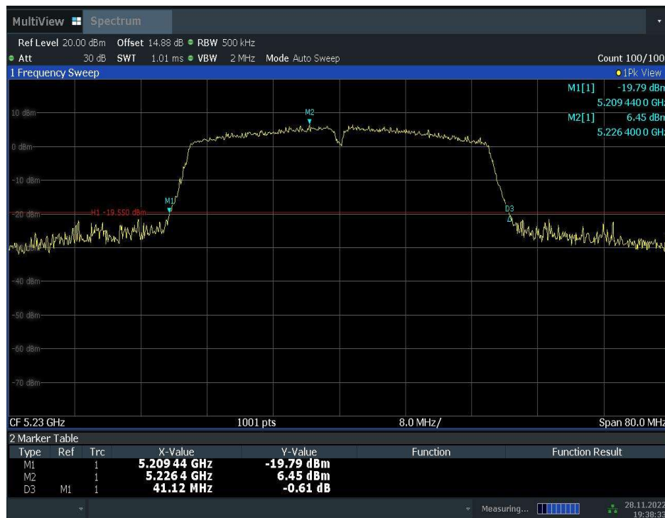
Fig.22 Occupied 26dB Bandwidth (802.11n-HT40, 5230MHz)
