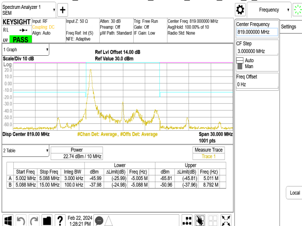
Emission Mask_Band26-Part90s_10MHz_QPSK_RB1_49_CH26740
