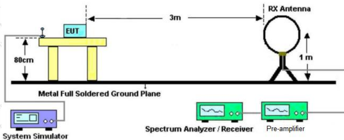
Figure 1. Below 30MHz
