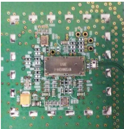
EUT – PCBA1 Component Side
