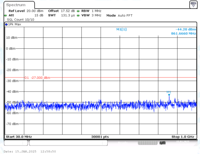
11N20-CDD-Ant2-5320-30~1000-PASS
