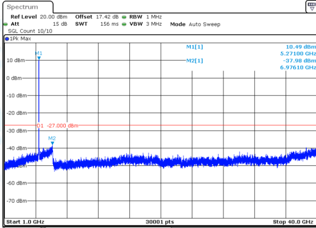
11N40-CDD-Ant1-5270-1000~40000-PASS
