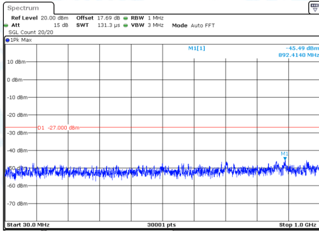
11N20-CDD-Ant1-5785-30~1000-PASS
