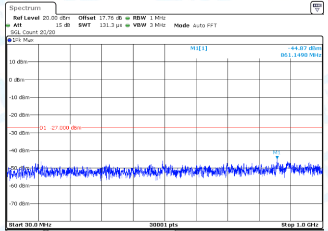
11N20-CDD-Ant2-5785-30~1000-PASS
