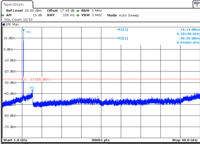
11N20-CDD-Ant1-5180-1000~40000-PASS
