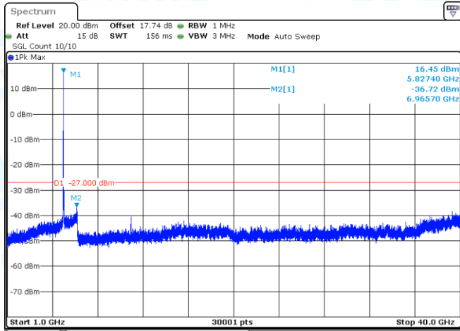
11N20-CDD-Ant1-5825-1000~40000-PASS
