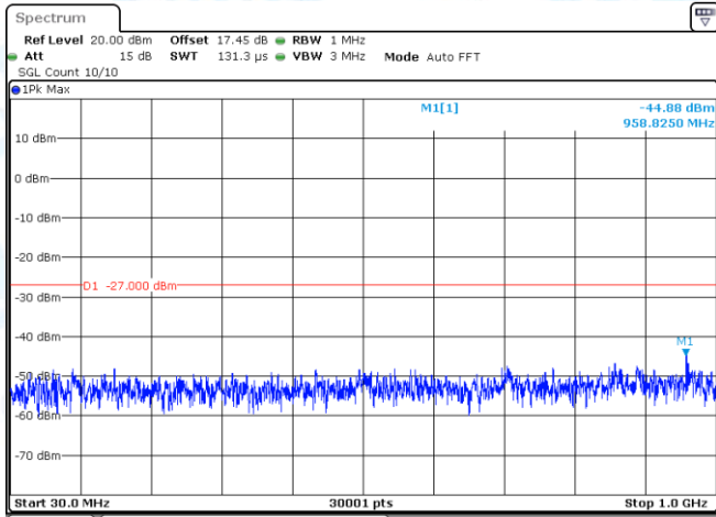
11AC20-CDD-Ant1-5180-30~1000-PASS
