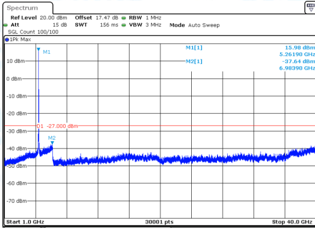
11N20-CDD-Ant1-5260-1000~40000-PASS
