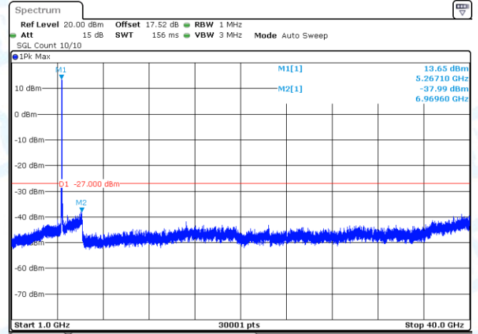
11N40-CDD-Ant2-5270-1000~40000-PASS
