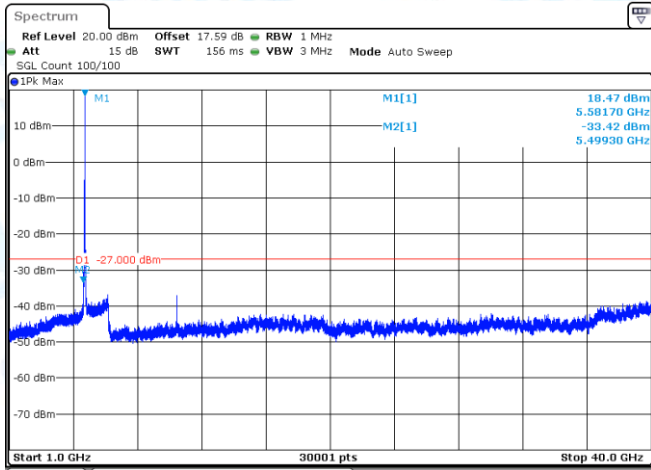
11A-Ant1-5580-1000~40000-PASS
