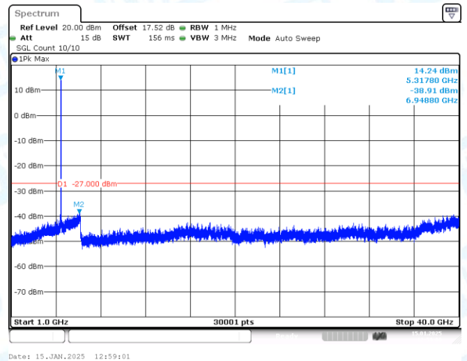
11N20-CDD-Ant2-5320-1000~40000-PASS
