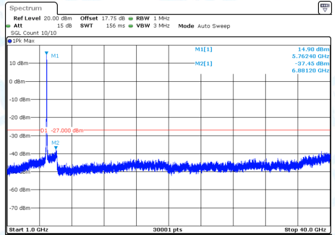
11N40-CDD-Ant2-5755-1000~40000-PASS
