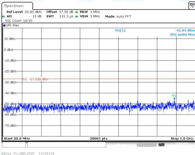
11N20-CDD-Ant1-5500-30~1000-PASS
