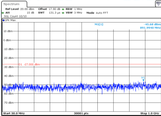
11N40-CDD-Ant1-5710-30~1000-PASS
