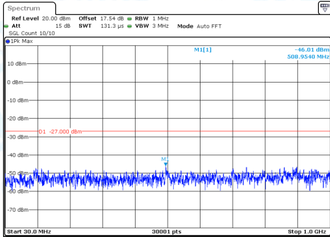
11N40-CDD-Ant1-5510-30~1000-PASS
