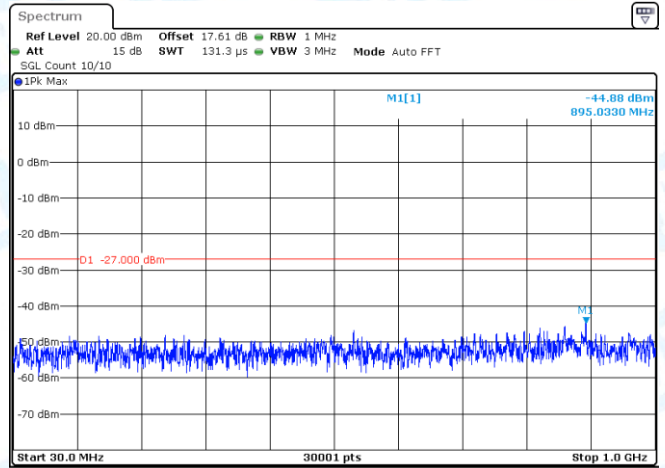
11N40-CDD-Ant2-5510-30~1000-PASS
