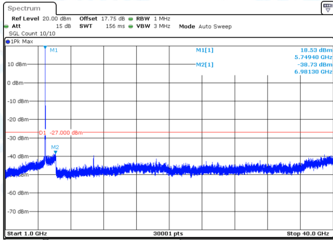
11A-Ant1-5745-1000~40000-PASS
