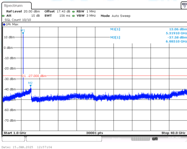
11N20-CDD-Ant1-5320-1000~40000-PASS
