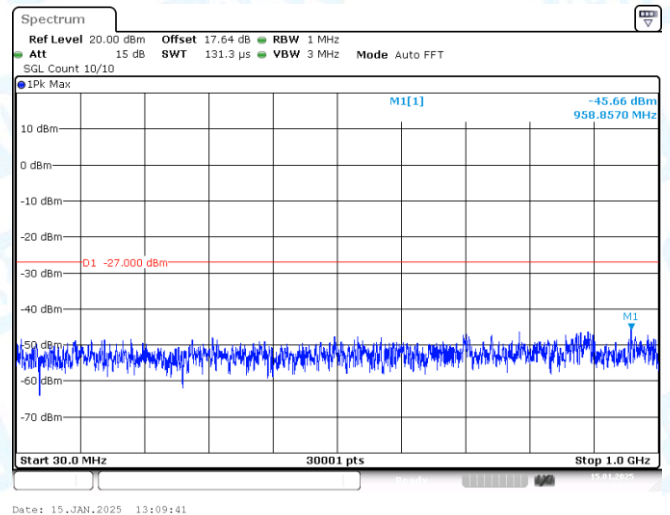
11N20-CDD-Ant2-5500-30~1000-PASS
