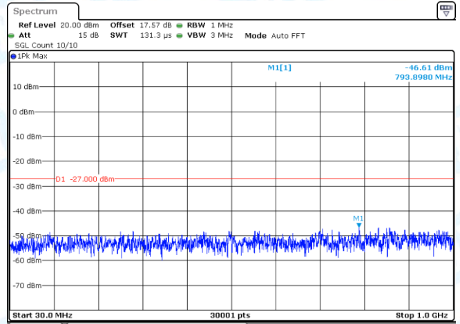
11N40-CDD-Ant2-5230-30~1000-PASS
