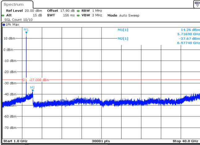
11N20-CDD-Ant1-5720-1000~40000-PASS
