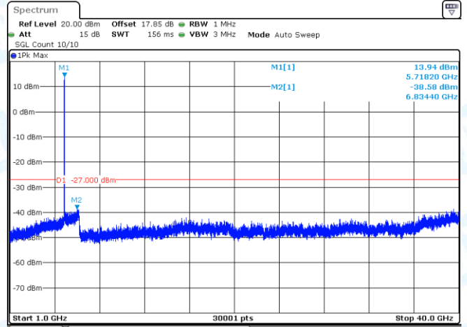
11N20-CDD-Ant2-5720-1000~40000-PASS
