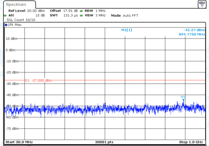
11N20-CDD-Ant2-5700-30~1000-PASS
