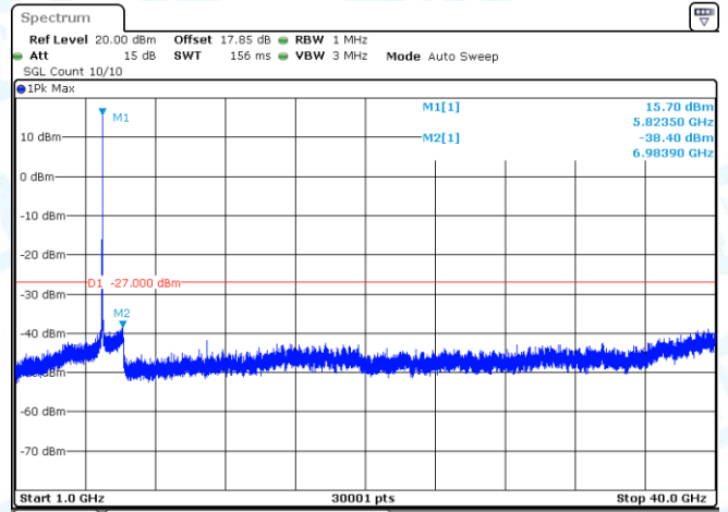
11N20-CDD-Ant2-5825-1000~40000-PASS
