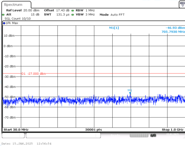
11N20-CDD-Ant1-5320-30~1000-PASS
