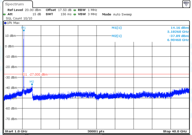
11N20-CDD-Ant2-5180-1000~40000-PASS
