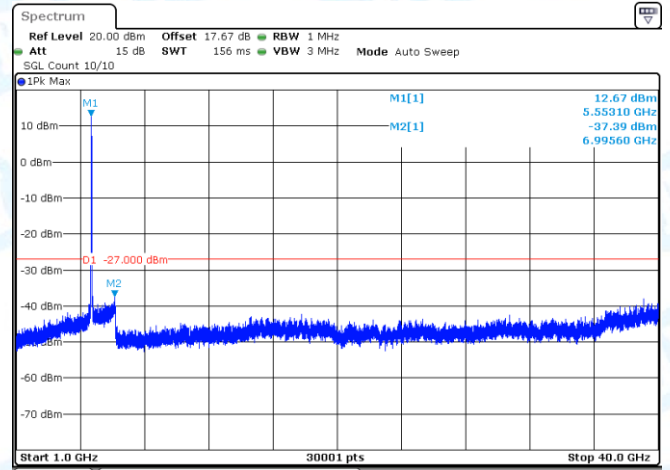
11N40-CDD-Ant2-5550-1000~40000-PASS
