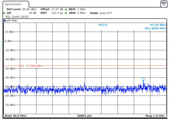
11N20-CDD-Ant2-5240-30~1000-PASS
