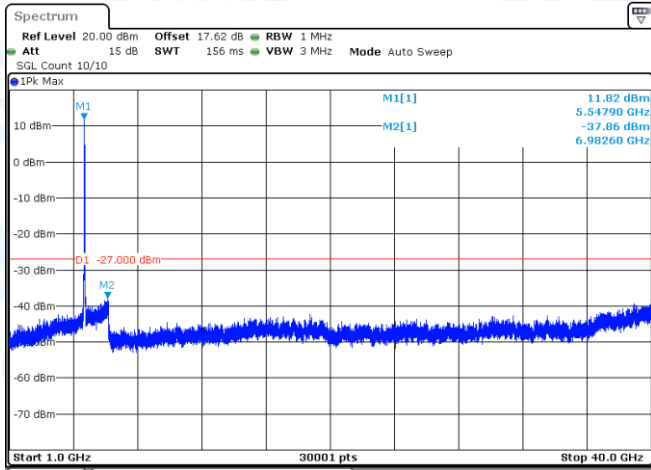
11N40-CDD-Ant1-5550-1000~40000-PASS
