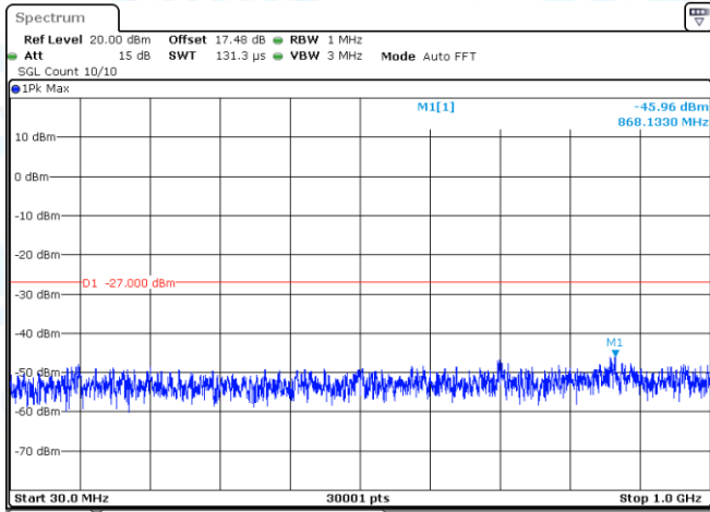
11N40-CDD-Ant1-5230-30~1000-PASS
