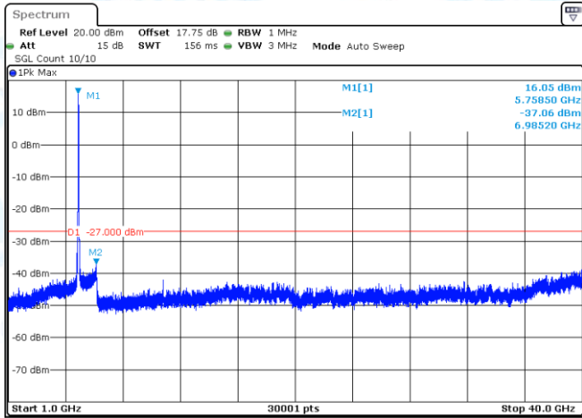
11N40-CDD-Ant1-5755-1000~40000-PASS
