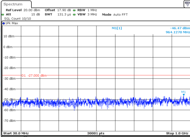
11N20-CDD-Ant1-5700-30~1000-PASS
