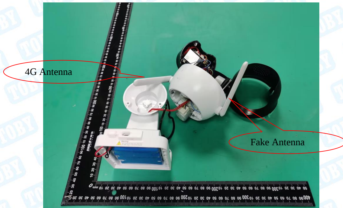
Photo 5 Internal of EUT
