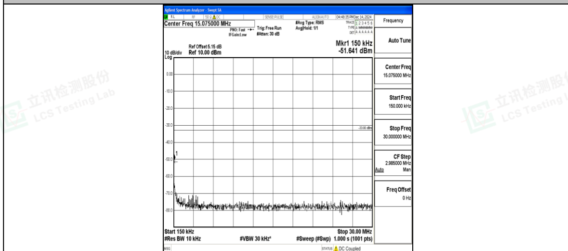
Band4_20MHz_QPSK_20175_1RB#0_0.15~30_0.15~30
