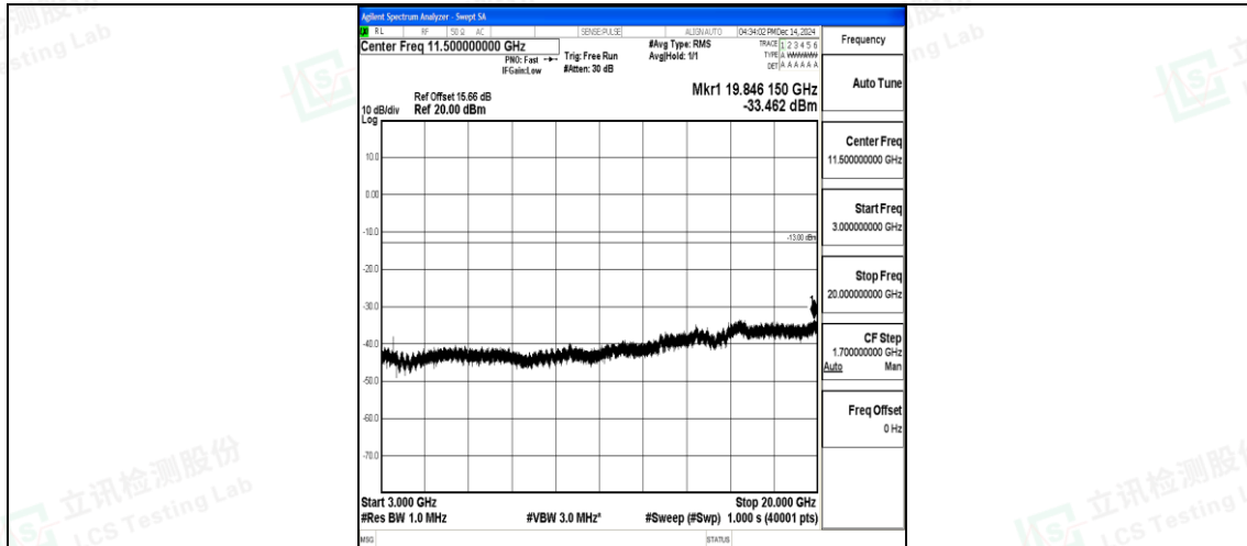
Band4_15MHz_QPSK_20325_1RB#0_3000~20000_3000~20000
