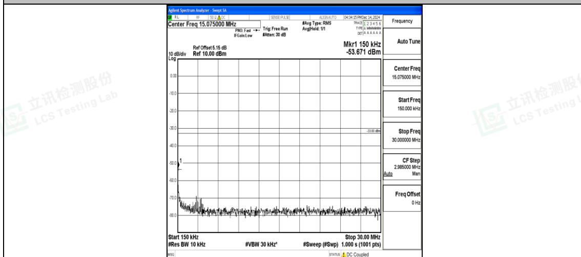
Band4_15MHz_16QAM_20325_1RB#0_0.15~30_0.15~30
