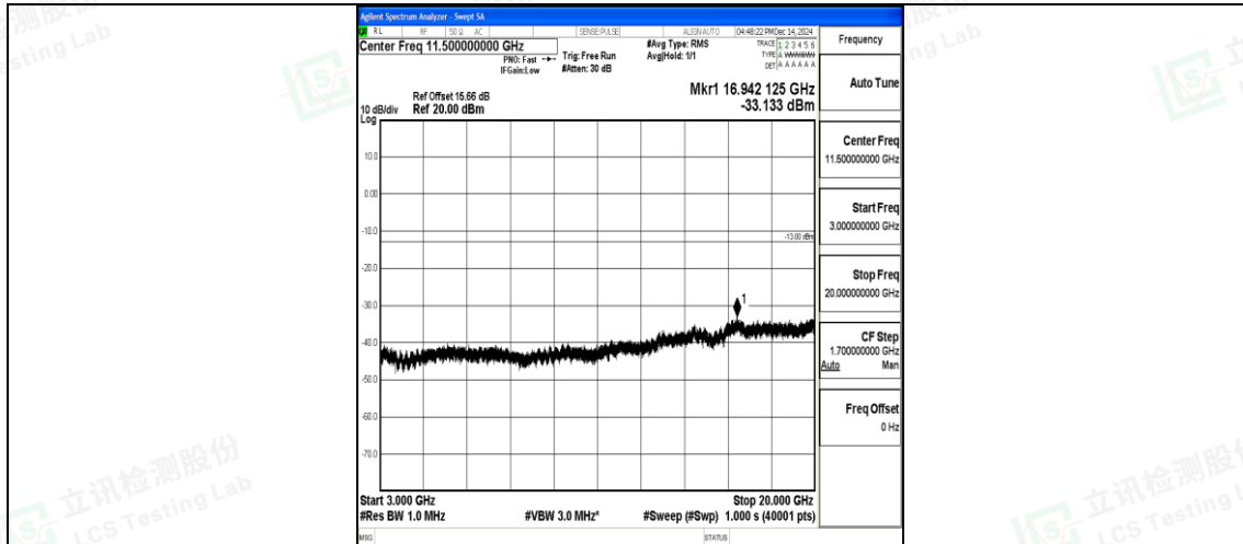
Band4_20MHz_16QAM_20050_1RB#0_3000~20000_3000~20000
