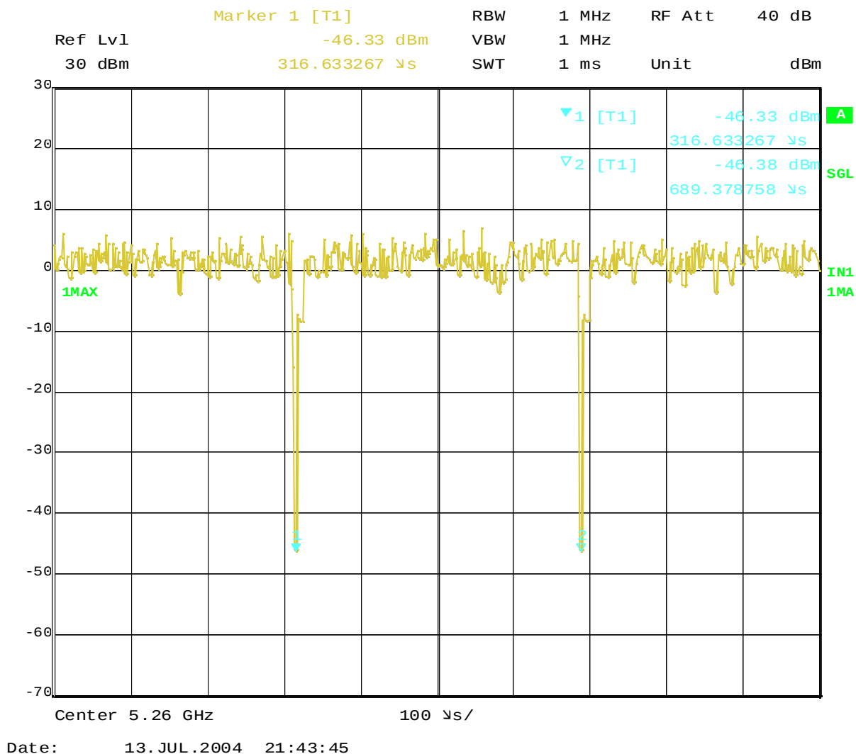
Plot 2-0 Transmission Pulse Duration
