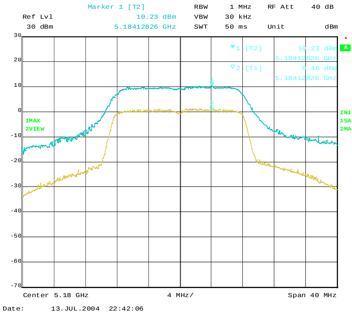
Plot 4-1 Peak Excursion Ratio at 5180MHz
