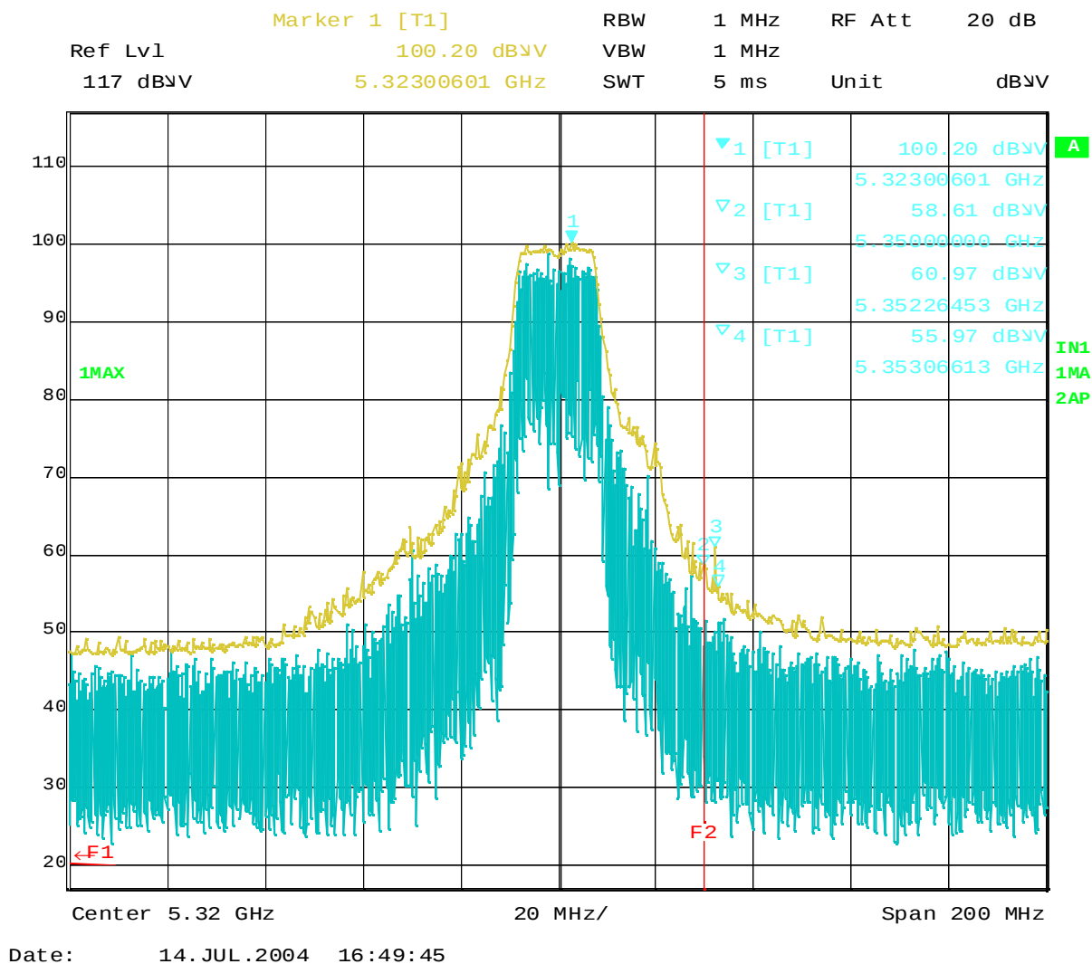
Plot 7-3 5320MHz TX mode (Peak). 14" model
