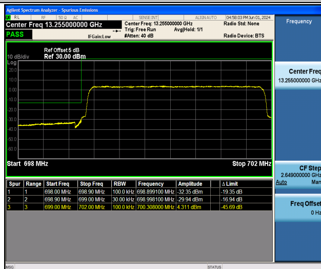
Band12_3MHz_16QAM_23025_15RB#0
