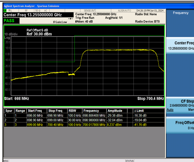
Band12_1.4MHz_16QAM_23017_6RB#0
