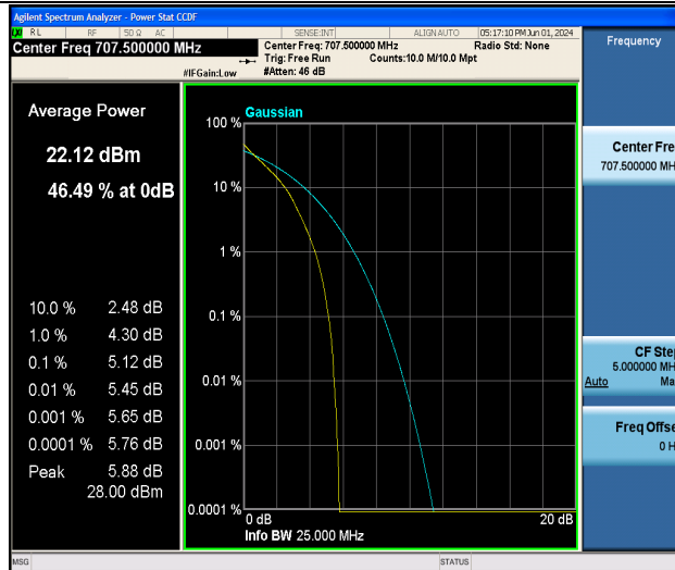
Band12-3MHz-QPSK-23095-15RB#0-PASS
