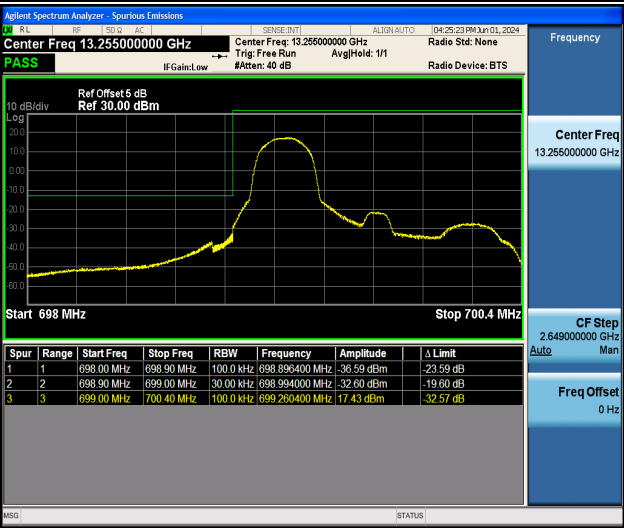
Band12_1.4MHz_16QAM_23017_1RB#0
