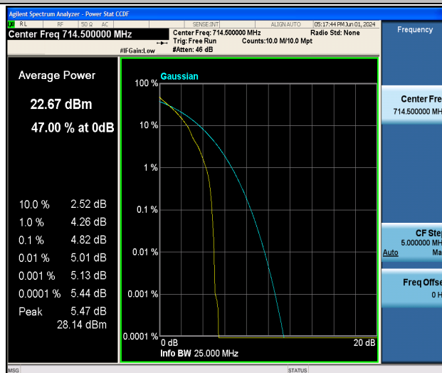
Band12-3MHz-QPSK-23165-1RB#0-PASS
