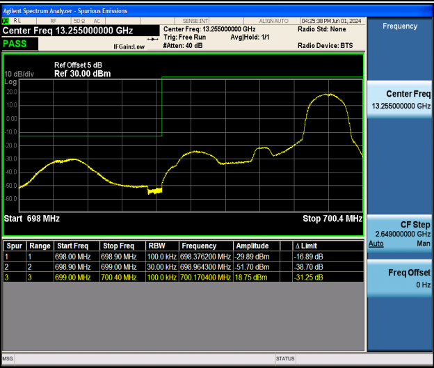
Band12_1.4MHz_QPSK_23017_1RB#5
