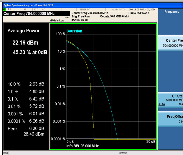
Band12-10MHz-16QAM-23060-1RB#0-PASS
