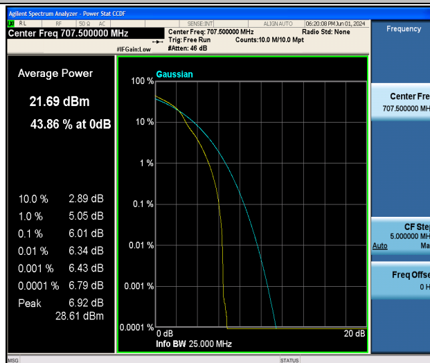
Band12-10MHz-16QAM-23095-1RB#0-PASS
