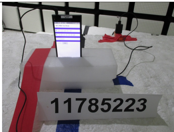
Z-AXIS ORIENTATION
