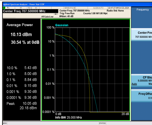
Band12-5MHz-QPSK-23095-6-0-Low-8.84-&lt;=13-PASS
