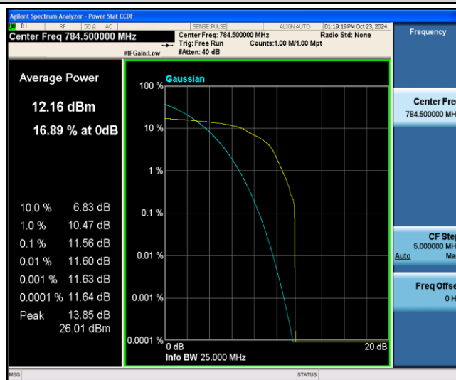
Band13-5MHz-16QAM-23255-1-0-Low-11.56-&lt;=13-PASS
