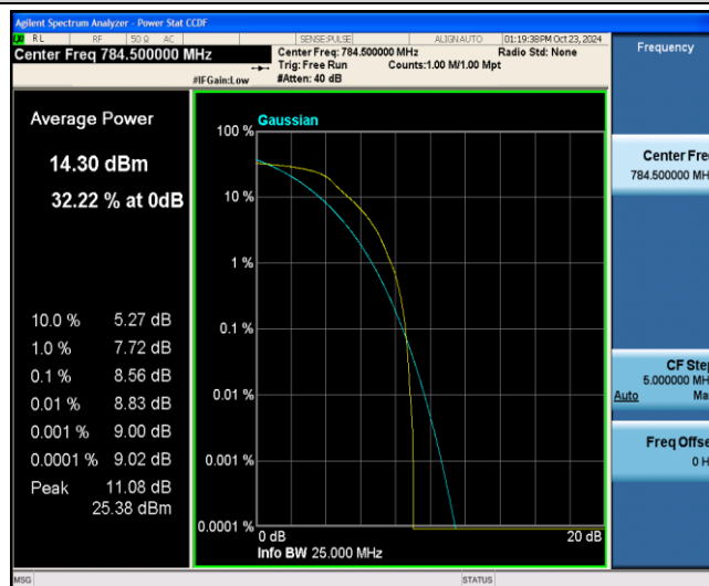
Band13-5MHz-16QAM-23255-6-0-Low-8.56-&lt;=13-PASS
