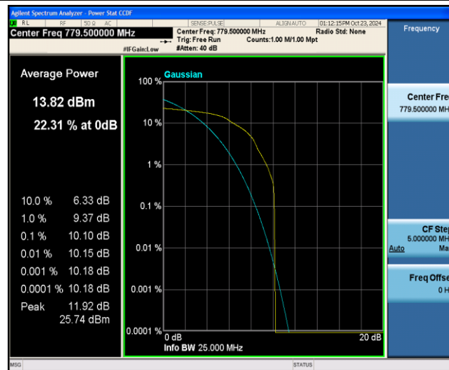
Band13-5MHz-16QAM-23205-1-0-Low-10.10-13-PASS
