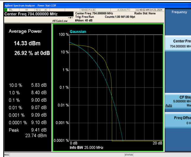
Band12-10MHz-QPSK-23060-1-0-Low-9.00-=&lt;=13-PASS
