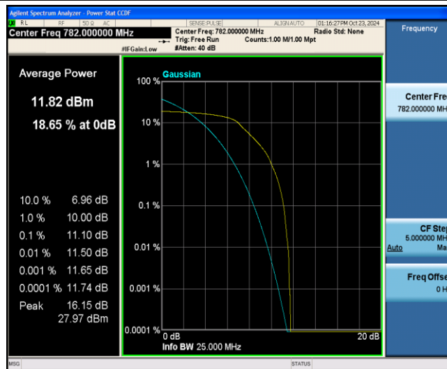
Band13-5MHz-QPSK-23230-6-0-Low-11.10-&lt;=13-PASS
