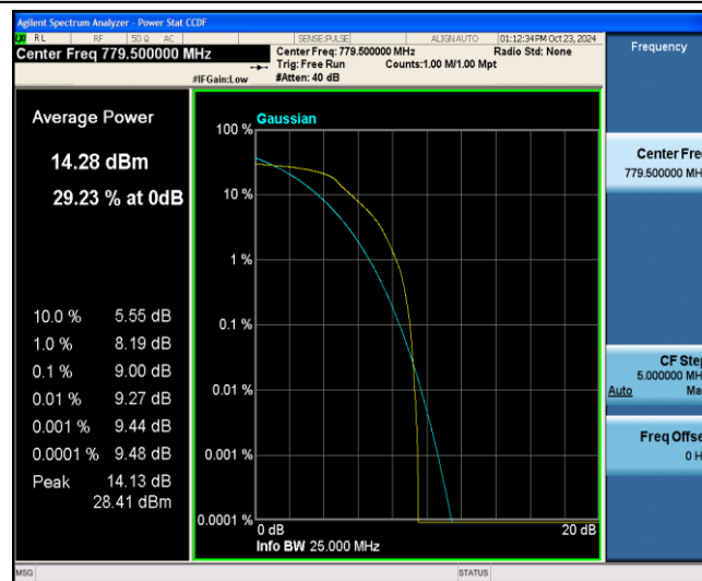
Band13-5MHz-16QAM-23205-6-0-Low-9.00-13-PASS
