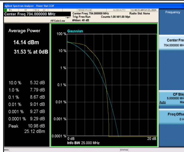
Band12-10MHz-QPSK-23060-6-0-Low-8.67-=&lt;=13-PASS
