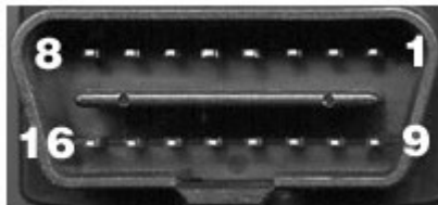
Connector on LMU3040LVB side
