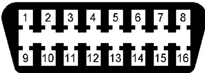
Connector on LMU3040LVB side
