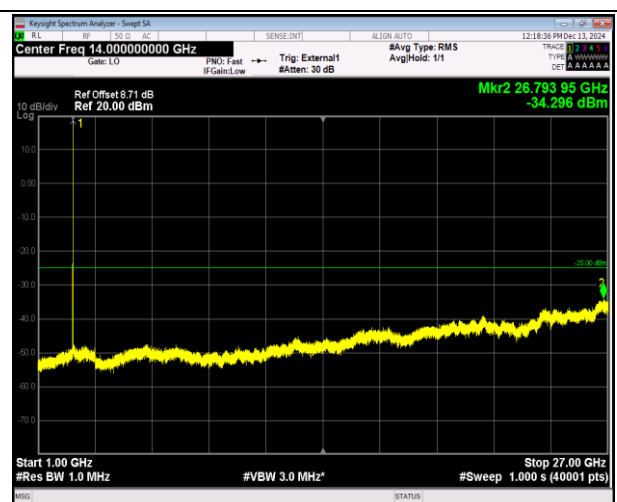
38-38-15MHz-15MHz-16QAM-16QAM-37925-38075-1RB# 74-ORB#0-1000~27000MHz-PASS
