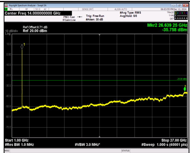
7-7-20MHz-10MHz-16QAM-16QAM-21051-21195-100RB#0 -50RB#0-1000~27000MHz-PASS
