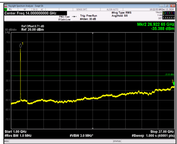
7-7-20MHz-20MHz-16QAM-16QAM-20850-21048-100RB# 0-100RB#0-1000~27000MHz-PASS
