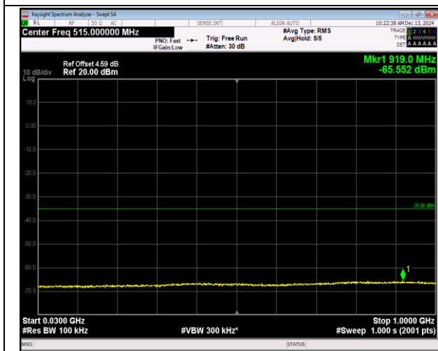
7-7-20MHz-20MHz-16QAM-16QAM-20850-21048-100RB #0-100RB#0-30~1000MHz-PASS
