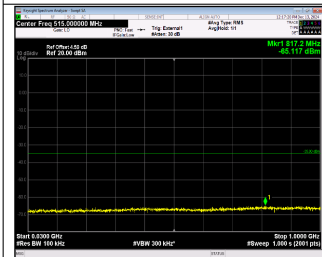
38-38-15MHz-15MHz-QPSK-QPSK-37925-38075-1RB#74-0RB#0-30~1000MHz-PASS
