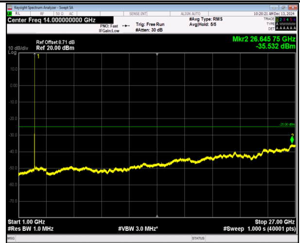
7-7-20MHz-20MHz-16QAM-16QAM-20850-21048-1RB#99- 0RB#0-1000~27000MHz-PASS
