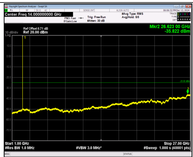
7-7-20MHz-10MHz-16QAM-16QAM-21251-21395-1RB#99- 0RB#0-1000~27000MHz-PASS
