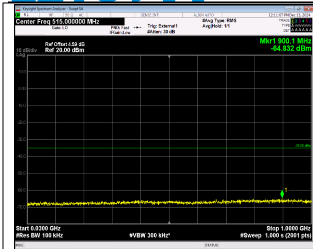
38-38-15MHz-15MHz-16QAM-16QAM-37825-37975-1RB #74-0RB#0-30~1000MHz-PASS
