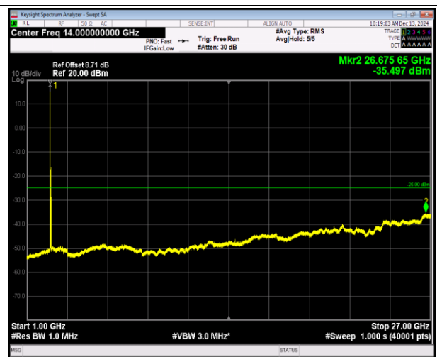
7-7-20MHz-20MHz-16QAM-16QAM-20850-21048-1RB#0-0RB#0-1000~27000MHz-PASS
