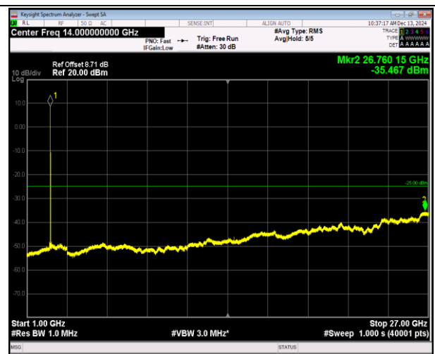
7-7-20MHz-20MHz-16QAM-16QAM-21001-21199-1RB#0-1 RB#99-1000~27000MHz-PASS
