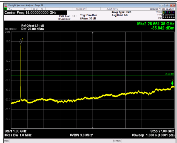
7-7-20MHz-10MHz-16QAM-16QAM-21251-21395-100RB# 0-50RB#0-1000~27000MHz-PASS
