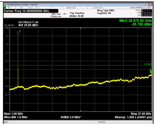
7-7-20MHz-10MHz-QPSK-QPSK-21251-21395-1RB#0-1RB #49-1000~27000MHz-PASS
