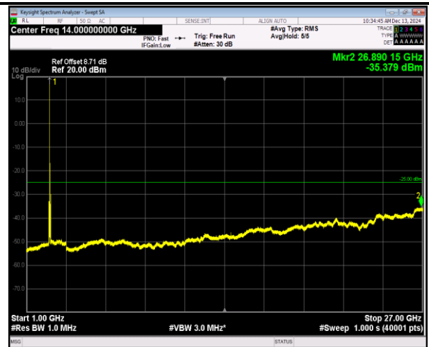
7-7-20MHz-20MHz-16QAM-16QAM-21001-21199-1RB#0-0 RB#0-1000~27000MHz-PASS
