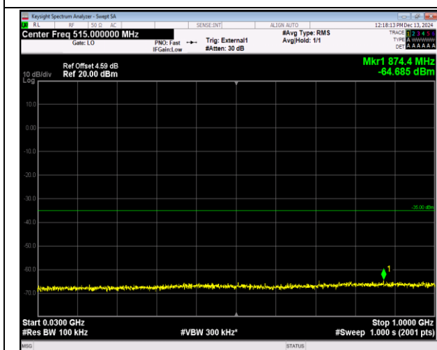
38-38-15MHz-15MHz-16QAM-16QAM-37925-38075-1RB #74-ORB#0-30~1000MHz-PASS
