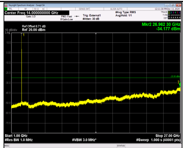
38-38-15MHz-15MHz-16QAM-16QAM-37825-37975-1RB# 74-0RB#0-1000~27000MHz-PASS
