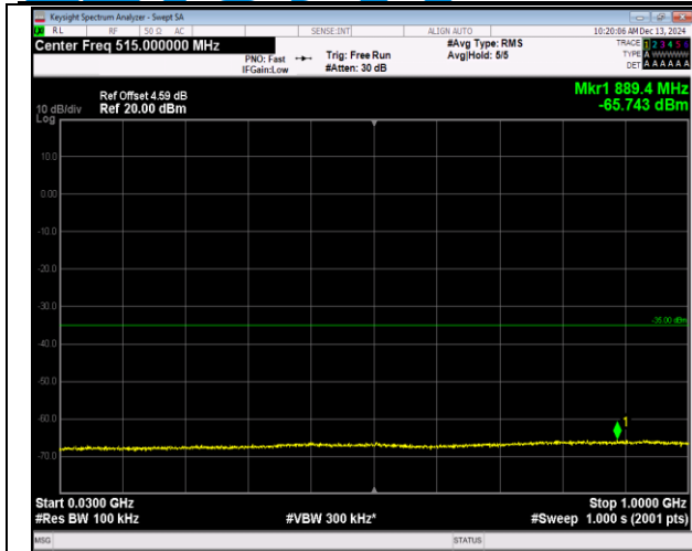
7-7-20MHz-20MHz-16QAM-16QAM-20850-21048-1RB#9 9-0RB#0-30~1000MHz-PASS
