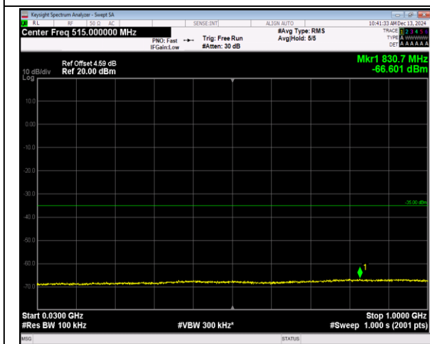
7-7-20MHz-20MHz-QPSK-QPSK-21152-21350-1RB#0-1 RB#99-30~1000MHz-PASS
