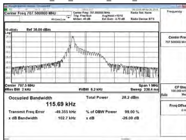
B12_15K_CH23095_BPSK_1RB0
