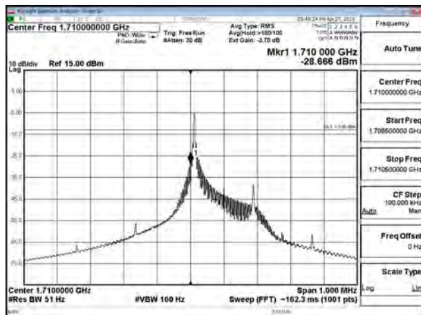
B4_3.75K_CH19951_BPSK_1RB0
