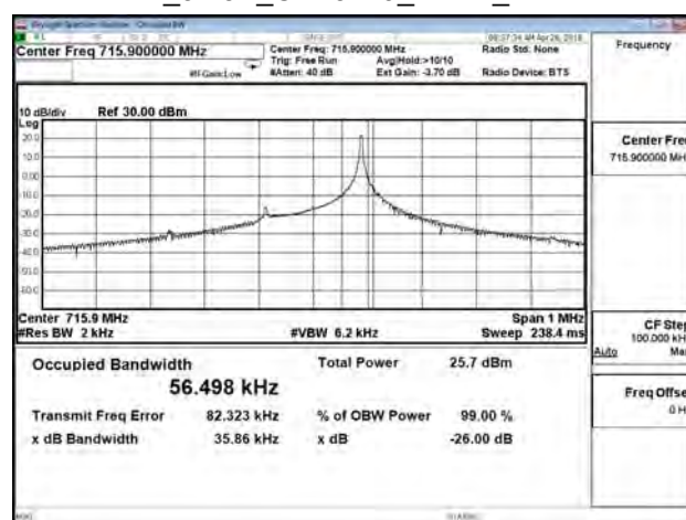
B12_3.75K_CH23179_BPSK_1RB47
