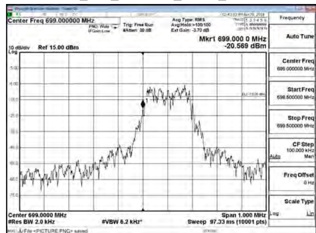
B12_15K_CH23011_QPSK_12RB0
