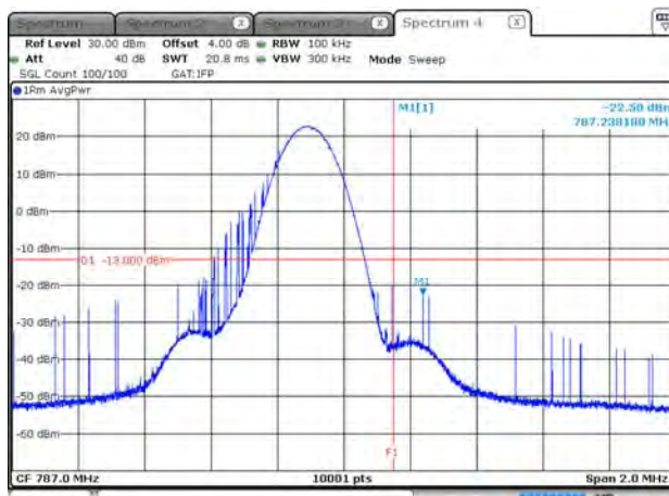
B13_3.75K_CH23278_BPSK_1RB47_150k
