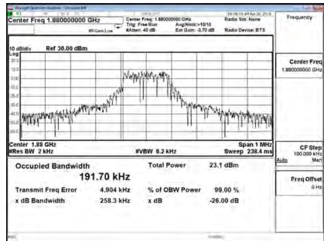
B2_15K_CH18900_QPSK_12RB0
