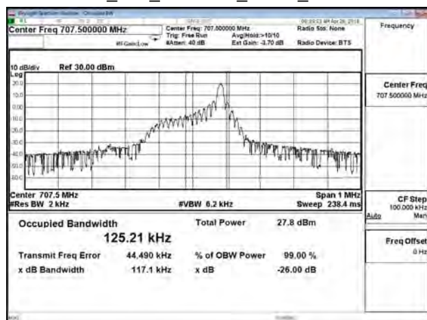
B12_15K_CH23095_QPSK_1RB11
