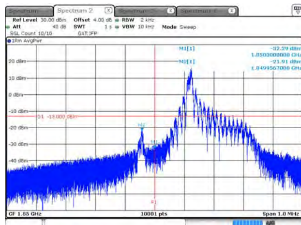
B2_15K_CH18602_QPSK_1RB0
