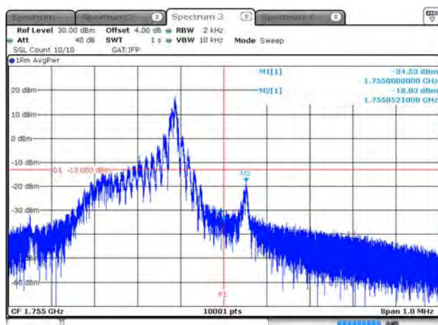
B4_15K_CH20398_QPSK_1RB11
