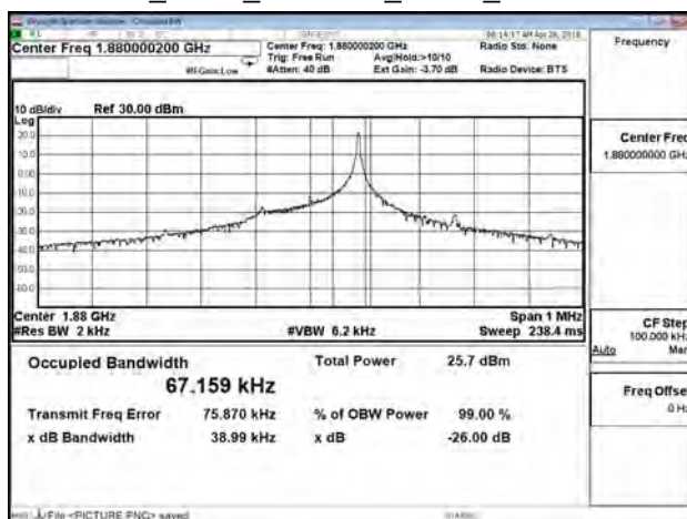
B2_3.75K_CH18900_QPSK_1RB47
