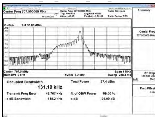
B12_15K_CH23095_BPSK_1RB11
