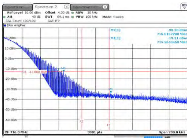
B12_3.75K_CH23178_QPSK_1RB47_15k
