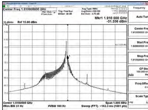
B2_3.75K_CH19199_BPSK_1RB47
