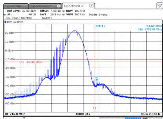
B12_3.75K_CH23178_QPSK_1RB47_150k
