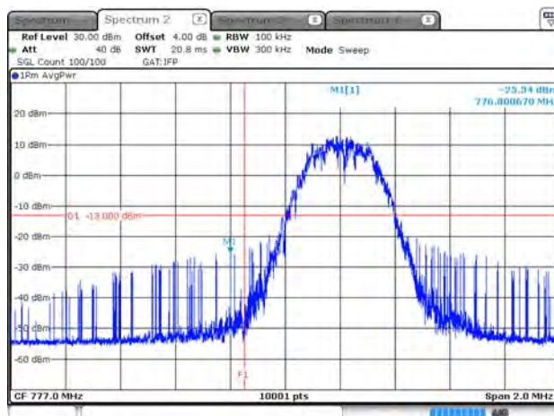
B13_15K_CH23182_QPSK_12RB0_150k
