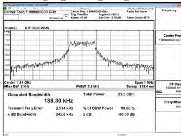
B2_15K_CH19199_QPSK_12RB0
