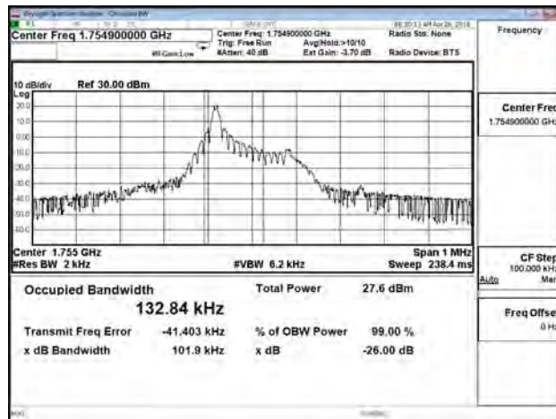
B4_15K_CH20399_BPSK_1RB0
