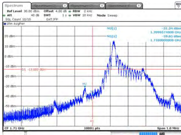
B4_15K_CH19952_BPSK_1RB0
