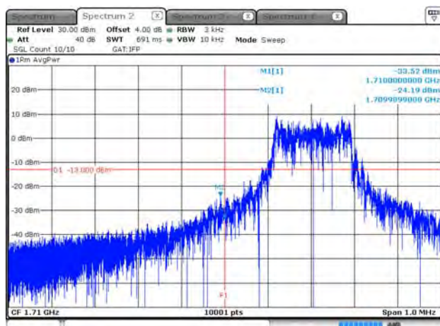
B4_15K_CH19952_QPSK_12RB0
