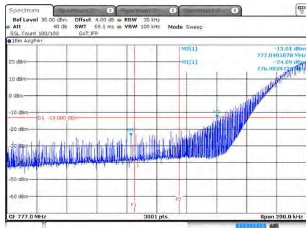
B13_3.75K_CH23182_BPSK_1RB0_15k
