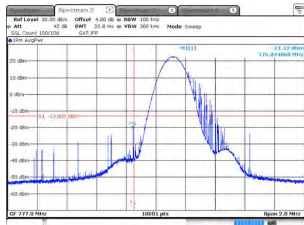
B13_3.75K_CH23182_BPSK_1RB0_150k
