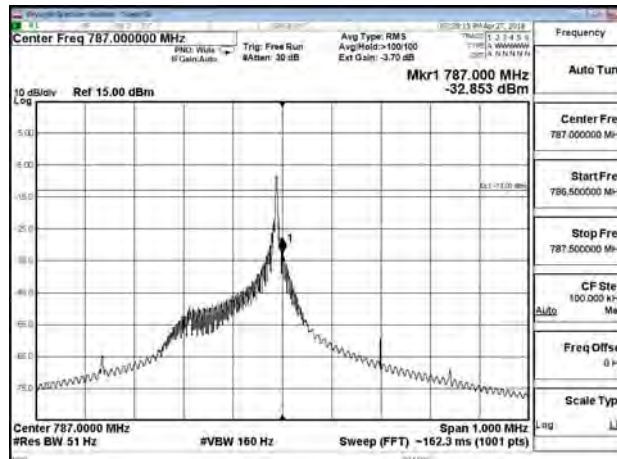
B13_3.75K_CH23279_QPSK_1RB47
