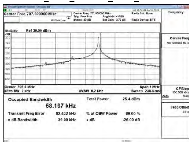
B12_3.75K_CH23095_BPSK_1RB47
