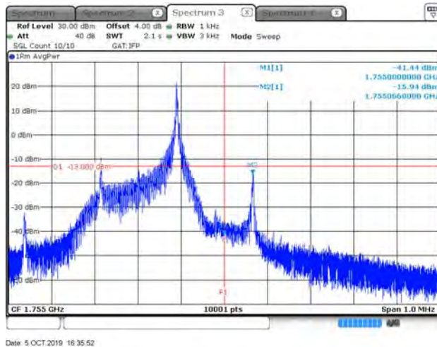
B4_3.75K_CH20398_BPSK_1RB47
