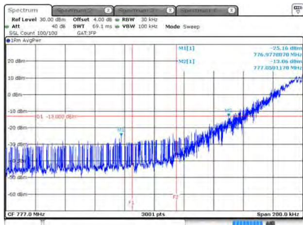
B13_15K_CH23182_QPSK_1RB0_15k
