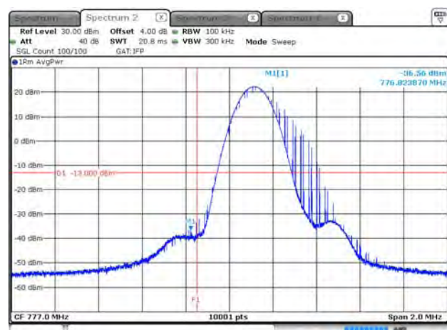
B13_3.75K_CH23182_QPSK_1RB0_150k
