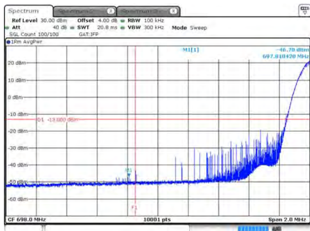
B12_15K_CH23011_BPSK_1RB0_150k
