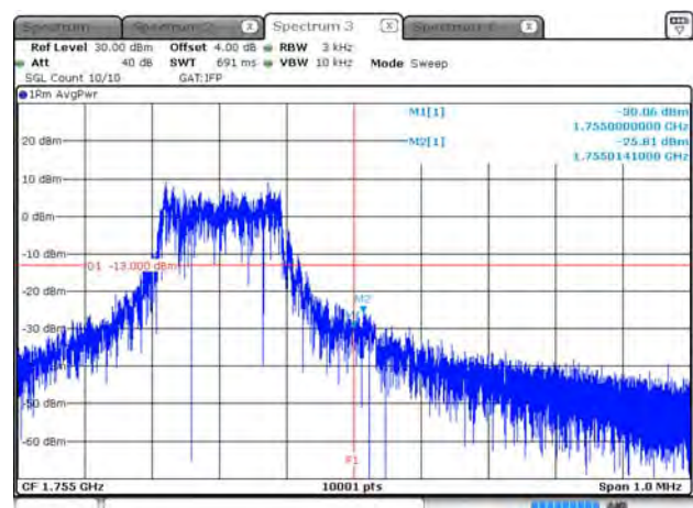
B4_15K_CH20398_QPSK_12RB0
