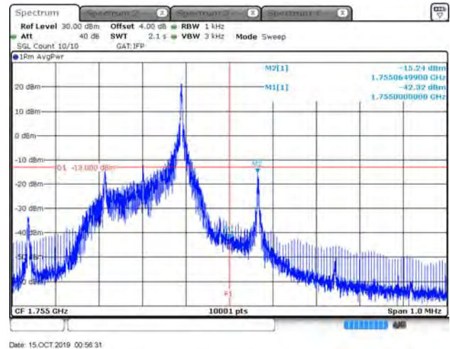
B4_3.75K_CH20398_QPSK_1RB47
