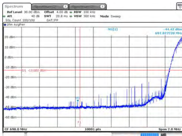
B12_15K_CH23011_QPSK_1RB0_150k
