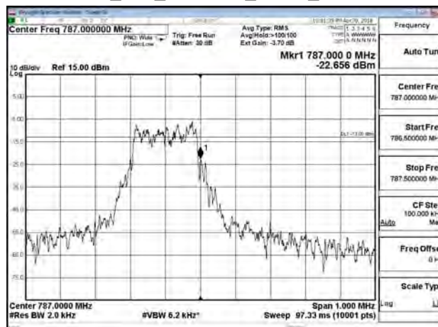
B13_15K_CH23279_QPSK_12RB0
