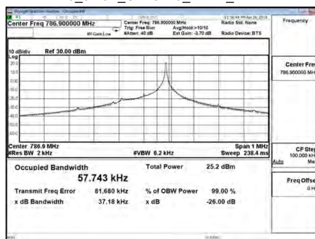
B13_3.75K_CH23279_BPSK_1RB47
