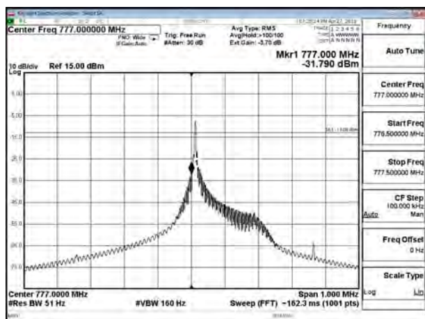
B13_3.75K_CH23181_QPSK_1RB0
