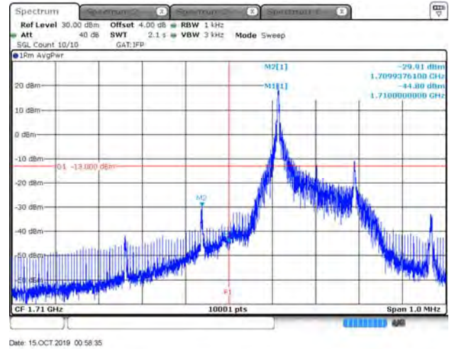
B4_3.75K_CH19952_QPSK_1RB0
