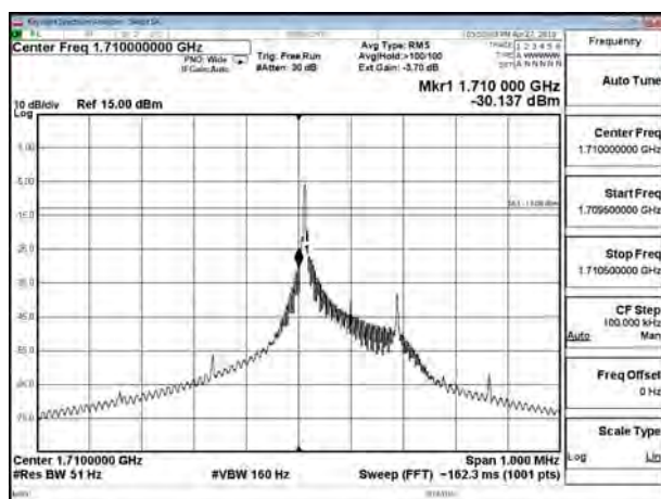
B4_3.75K_CH19951_QPSK_1RB0
