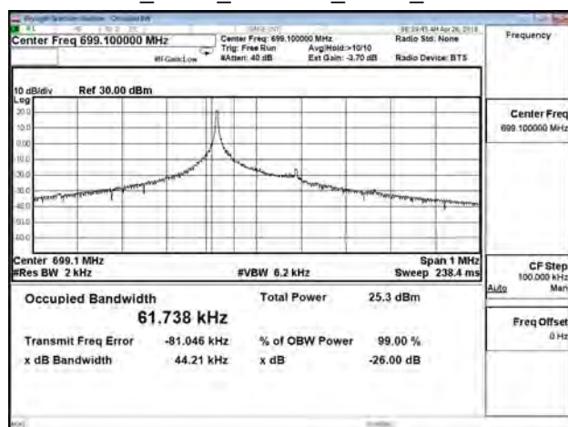
B12_3.75K_CH23011_BPSK_1RB0
