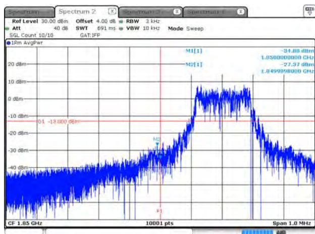
B2_15K_CH18602_QPSK_12RB0
