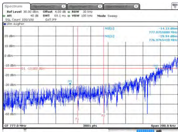
B13_15K_CH23182_QPSK_12RB0_15k
