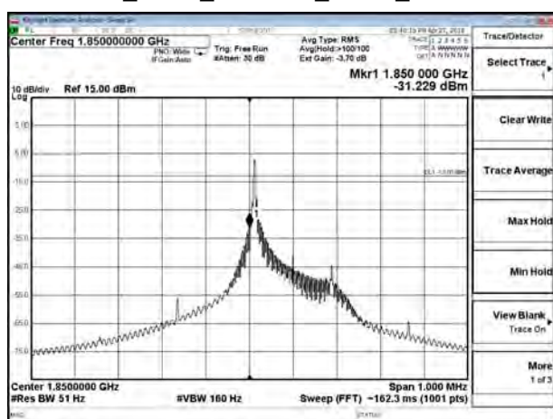
B2_3.75K_CH18601_QPSK_1RB0
