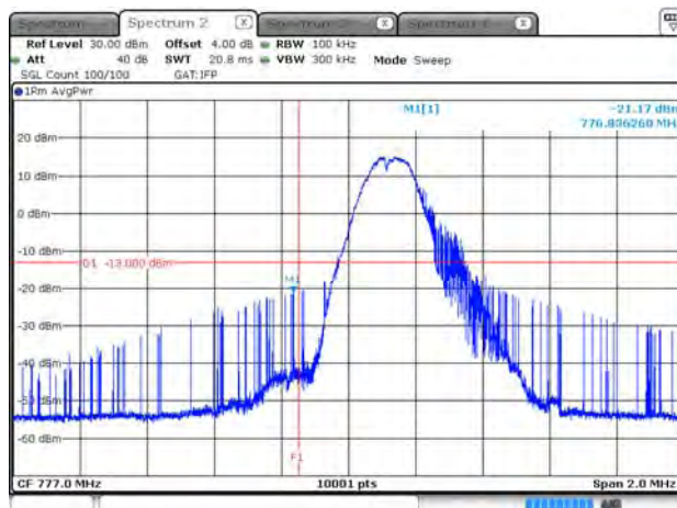
B13_15K_CH23182_QPSK_1RB0_150k
