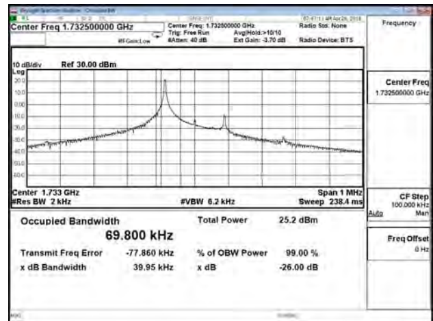
B4_3.75K_CH20175_BPSK_1RB0
