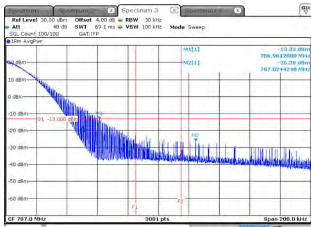
B13_3.75K_CH23278_BPSK_1RB47_15k
