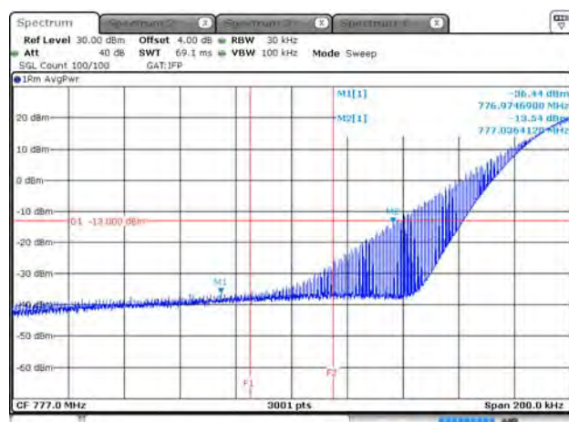
B13_3.75K_CH23182_QPSK_1RB0_15k
