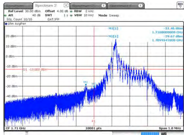
B4_15K_CH19952_QPSK_1RB0
