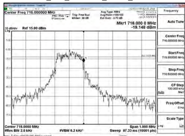
B12_15K_CH23179_QPSK_12RB0
