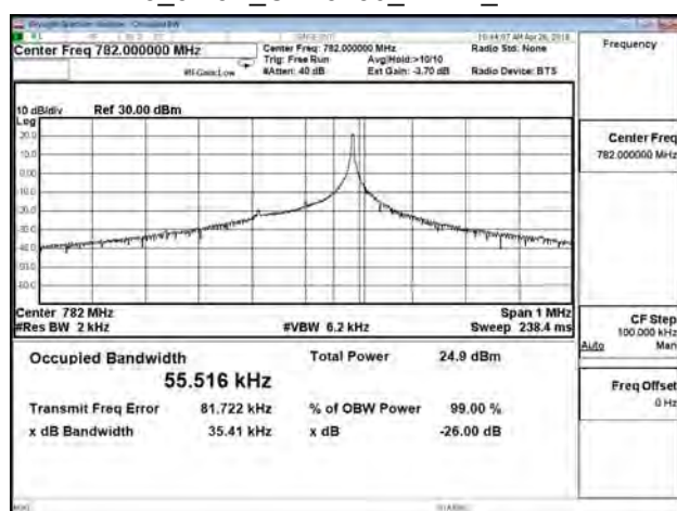
B13_3.75K_CH23230_BPSK_1RB47
