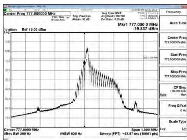
B13_15K_CH23181_QPSK_1RB0
