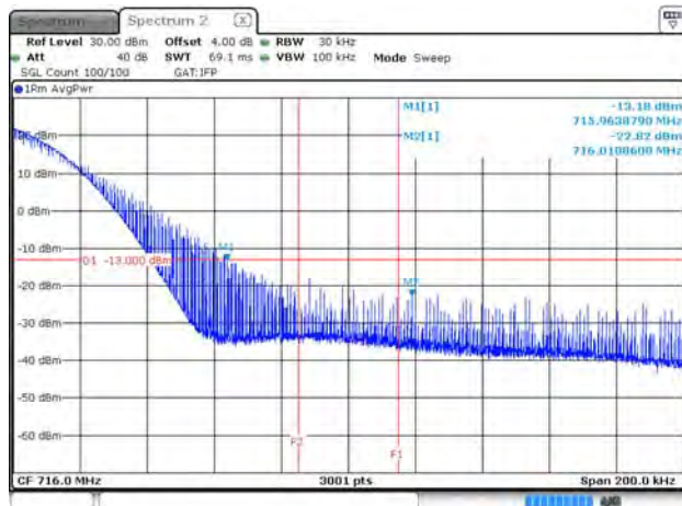
B12_3.75K_CH23178_BPSK_1RB47_15k
