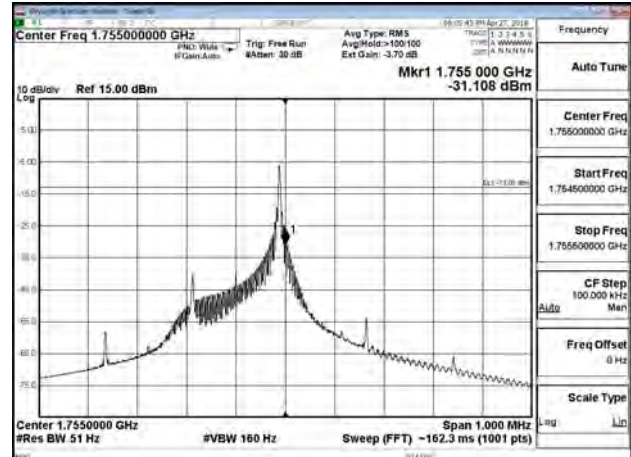
B4_3.75K_CH20399_BPSK_1RB47
