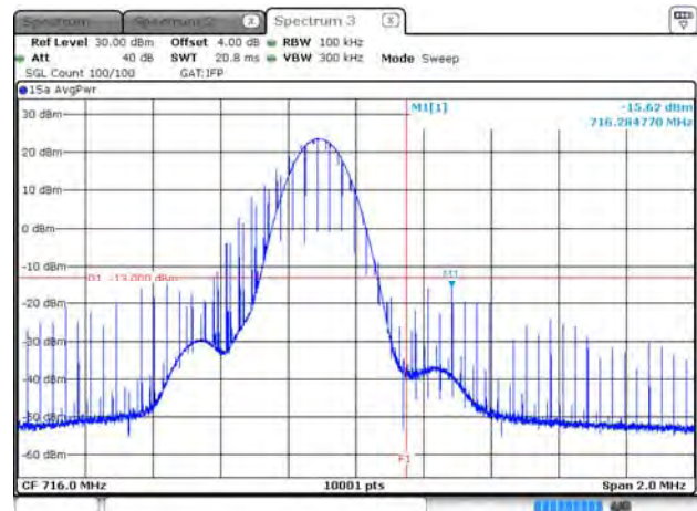
B12_3.75K_CH23178_BPSK_1RB47_150k
