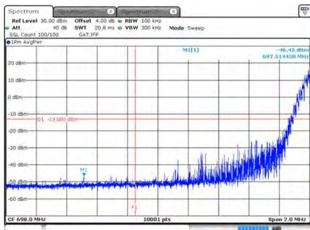
B12_15K_CH23011_QPSK_12RB0_150k
