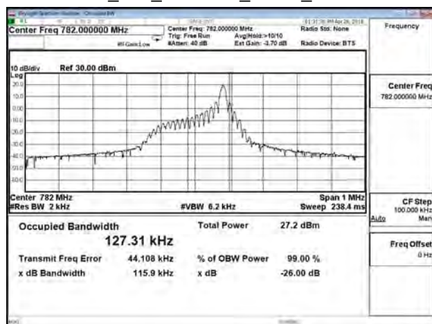
B13_15K_CH23230_QPSK_1RB11
