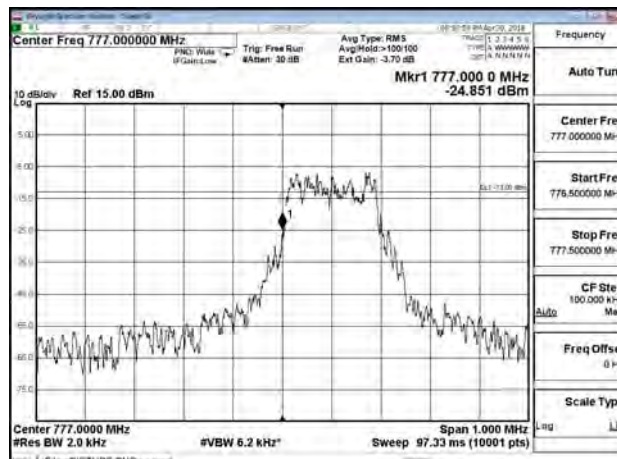
B13_15K_CH23181_QPSK_12RB0
