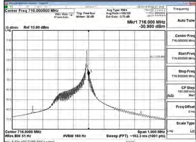
B12_3.75K_CH23179_BPSK_1RB47
