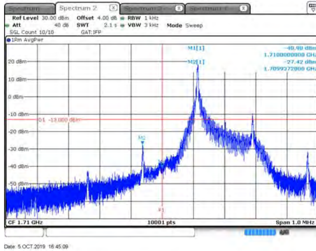
B4_3.75K_CH19952_BPSK_1RB0
