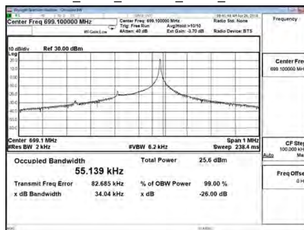
B12_3.75K_CH23011_BPSK_1RB47
