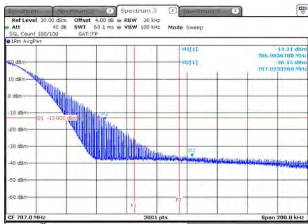
B13_3.75K_CH23278_QPSK_1RB47_15k
