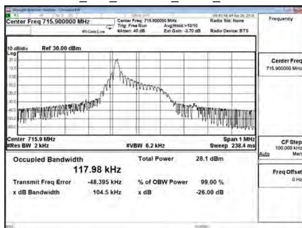
B12_15K_CH23179_BPSK_1RB0
