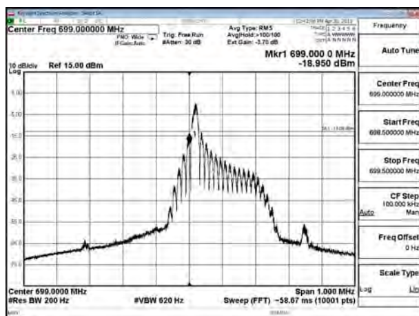
B12_15K_CH23011_QPSK_1RB0
