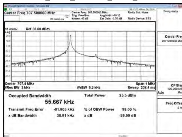
B12_3.75K_CH23095_BPSK_1RB0
