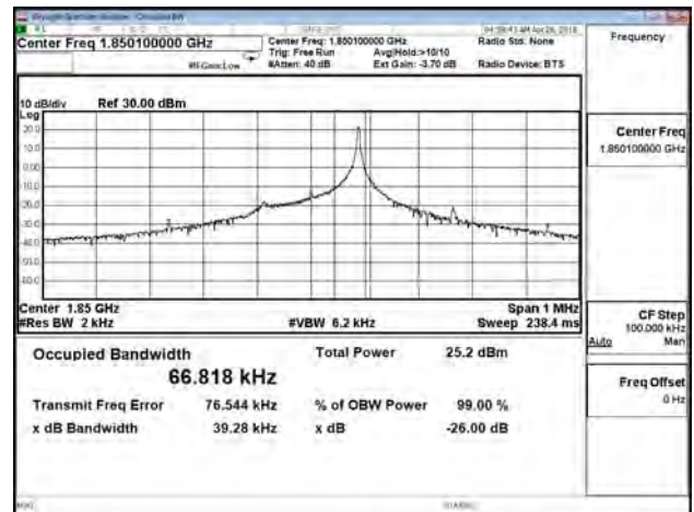
B2_3.75K_CH18601_QPSK_1RB47
