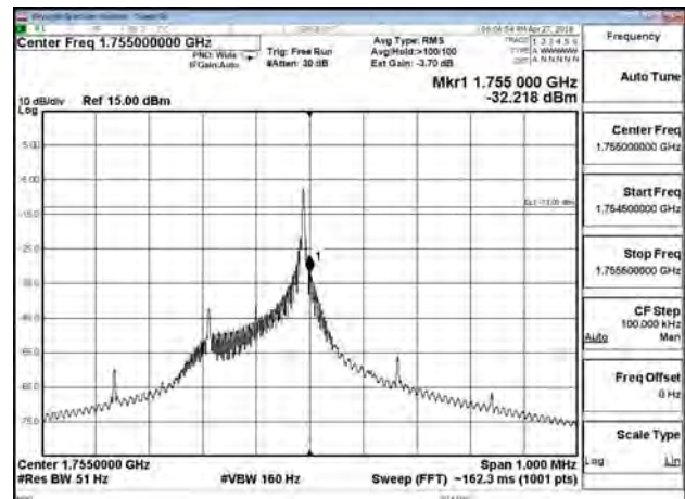
B4_3.75K_CH20399_QPSK_1RB47
