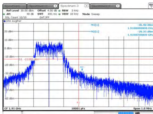
B2_15K_CH19198_QPSK_12RB0
