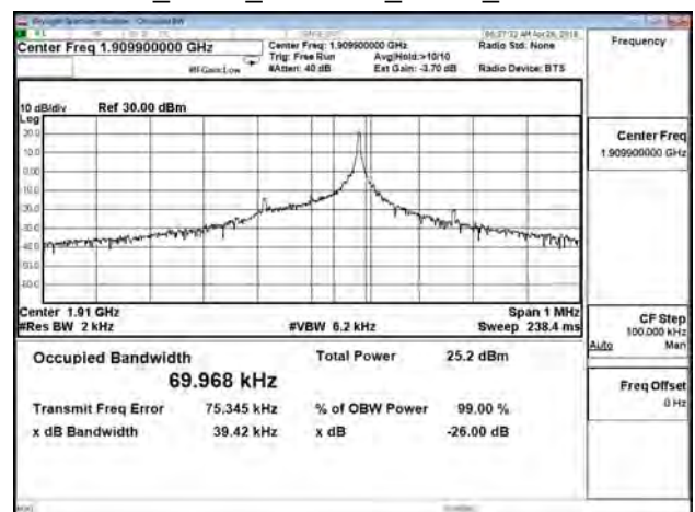
B2_3.75K_CH19199_QPSK_1RB47
