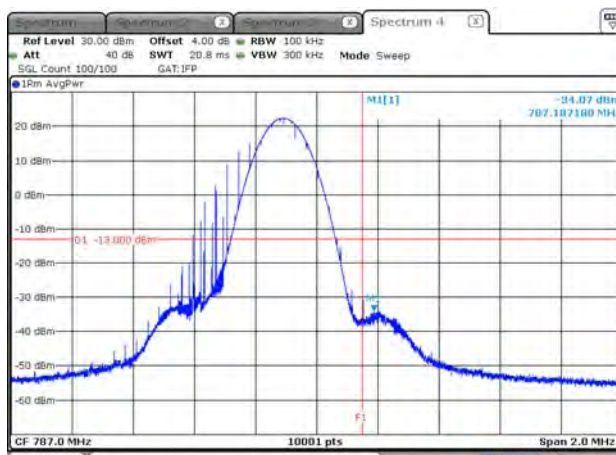
B13_3.75K_CH23278_QPSK_1RB47_150k
