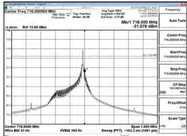
B12_3.75K_CH23179_QPSK_1RB47
