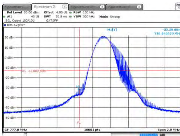
B13_15K_CH23182_BPSK_1RB0_150k
