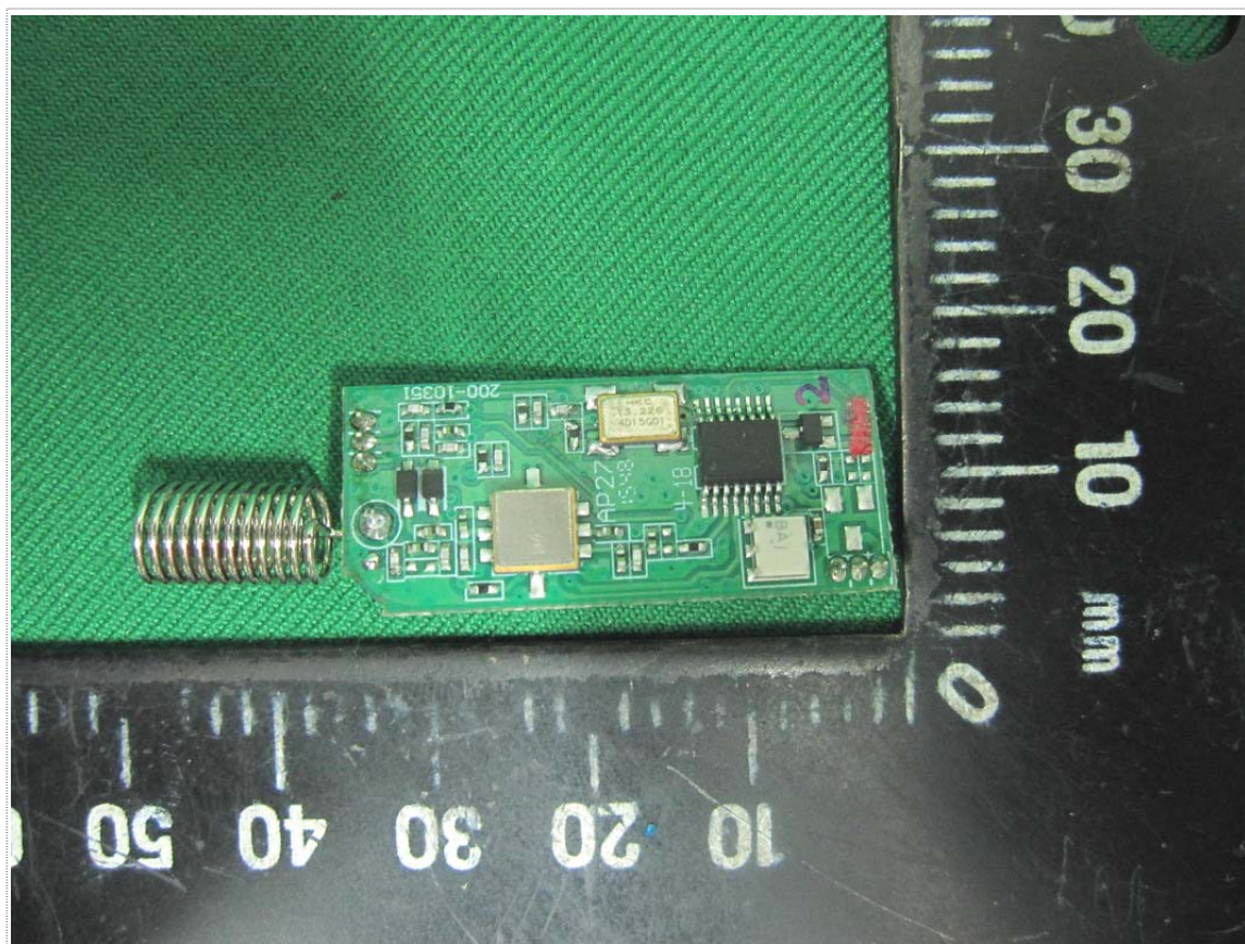
Front View of PCB-2
