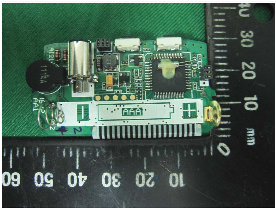
Front View of PCB-1
