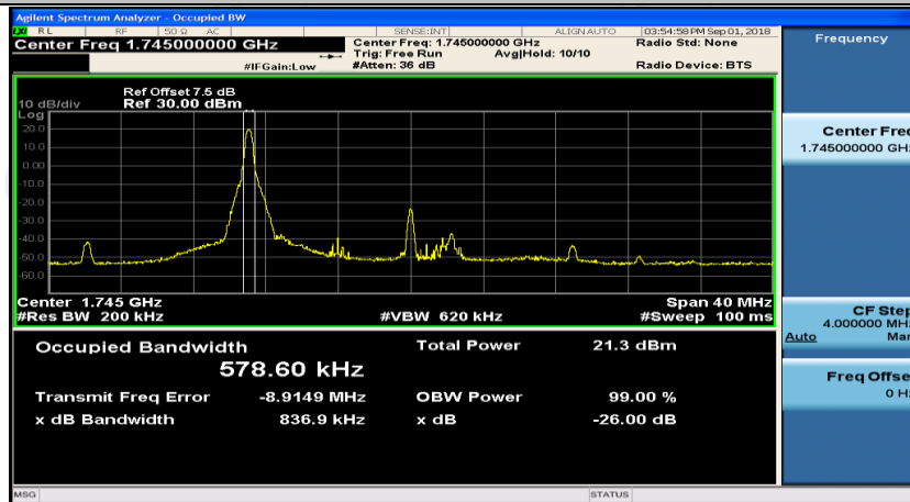
(Channel Bandwidth:20 MHz)_HCH_16QAM_1RB#50
