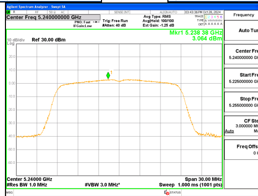
ANT L_802.11ac_VHT20_UNII 1
