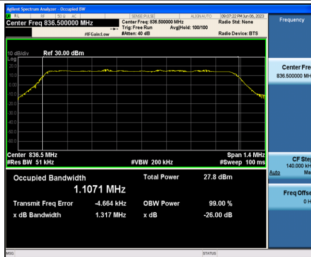
Band5-1.4MHz-QPSK-20525-6-0-Low-1.1071-1.317-PASS
