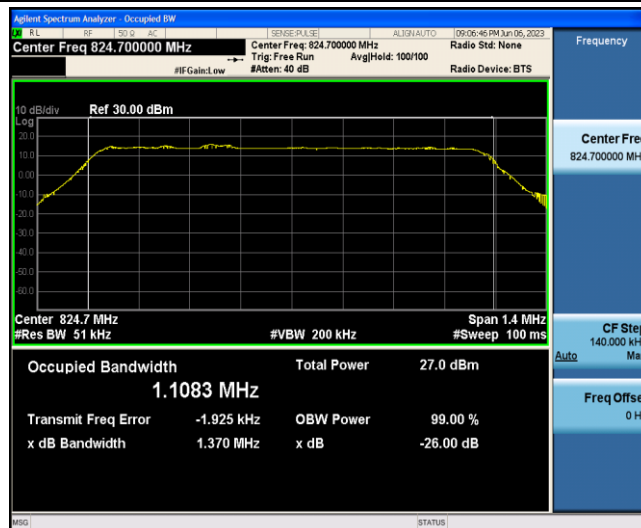
Band5-1.4MHz-QPSK-20407-6-0-Low-1.1083-1.370-PASS
