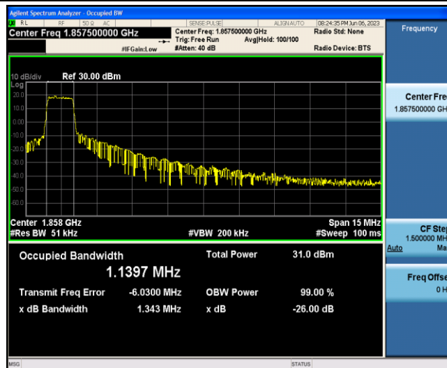
Band2-15MHz-QPSK-18675-6-0-Low-1.1397-1.343-PASS
