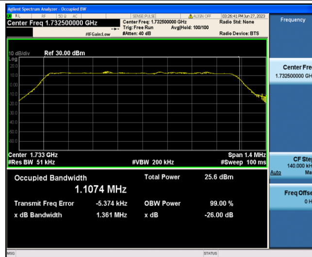
Band4-1.4MHz-QPSK-20175-6-0-Low-1.1074-1.361-PASS
