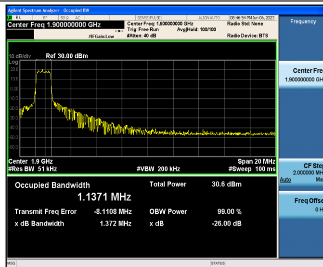
Band2-20MHz-16QAM-19100-6-0-Low-1.1371-1.372-PASS
