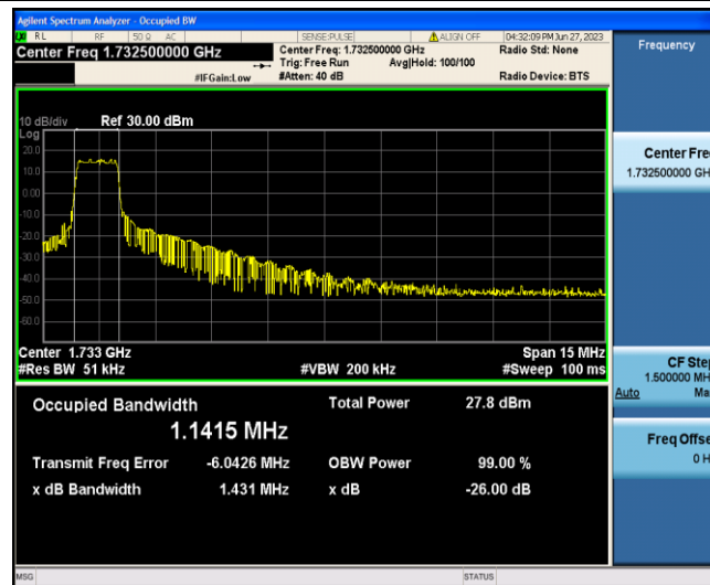
Band4-15MHz-QPSK-20175-6-0-Low-1.1415-1.431-PASS
