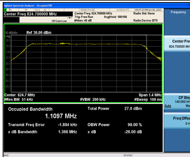
Band5-1.4MHz-16QAM-20407-6-0-Low-1.1097-1.366-PASS
