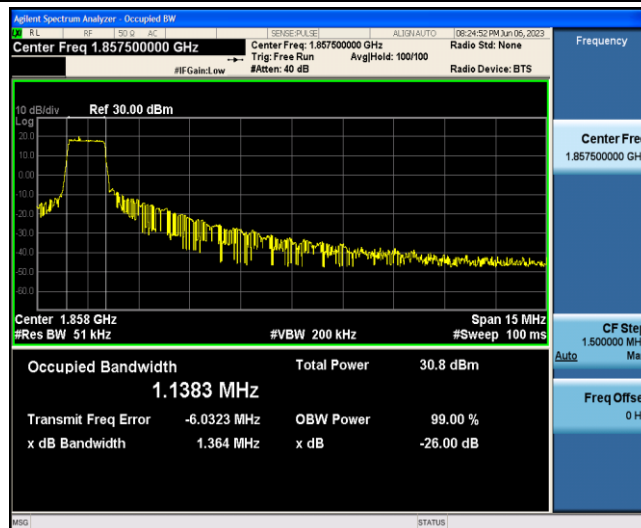
Band2-15MHz-16QAM-18675-6-0-Low-1.1383-1.364-PASS
