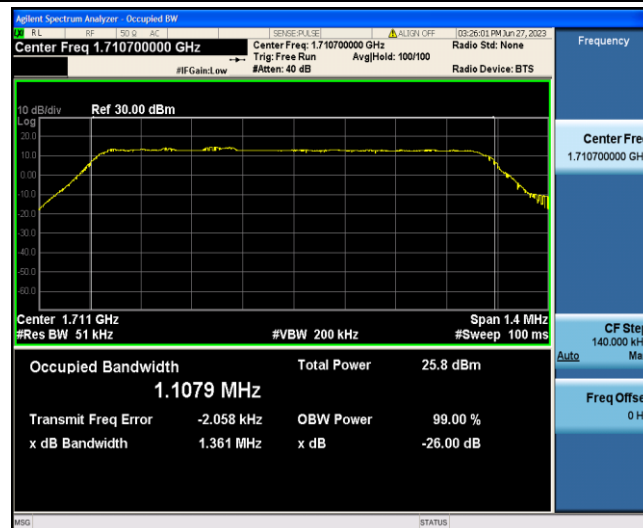
Band4-1.4MHz-QPSK-19957-6-0-Low-1.1079-1.361-PASS
