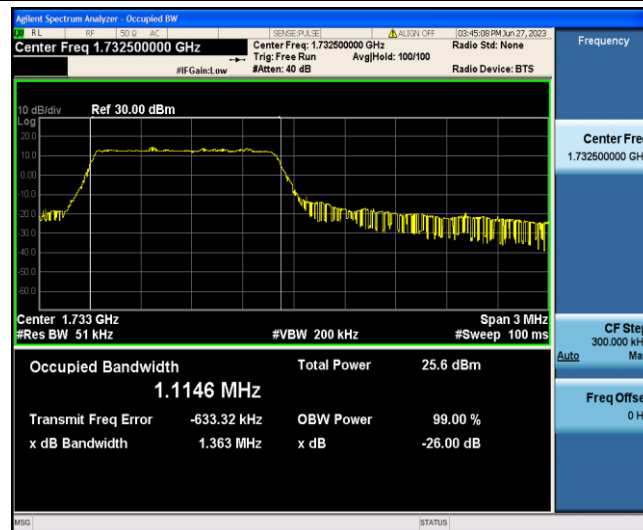
Band4-3MHz-16QAM-20175-6-0-Low-1.1146-1.363-PASS
