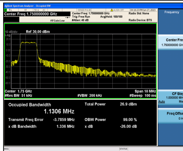
Band4-10MHz-16QAM-20350-6-0-Low-1.1306-1.336-PASS
