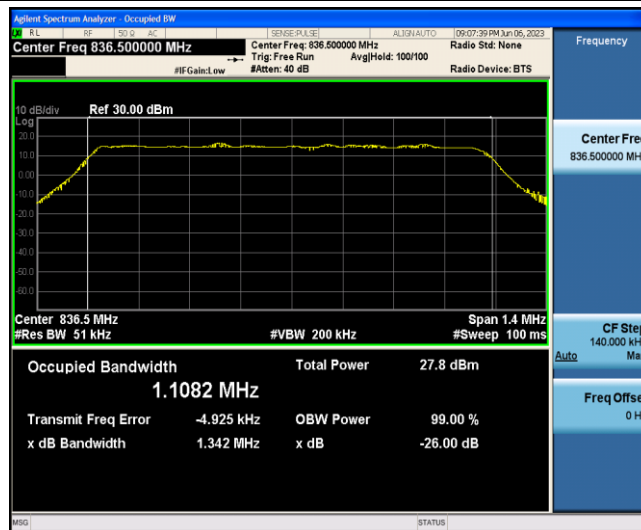
Band5-1.4MHz-16QAM-20525-6-0-Low-1.1082-1.342-PASS
