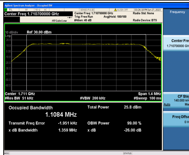
Band4-1.4MHz-16QAM-19957-6-0-Low-1.1084-1.359-PASS
