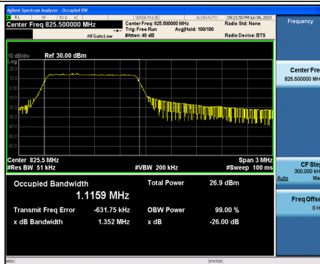
Band5-3MHz-QPSK-20415-6-0-Low-1.1159-1.352-PASS
