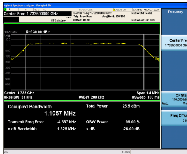
Band4-1.4MHz-16QAM-20175-6-0-Low-1.1057-1.325-PASS
