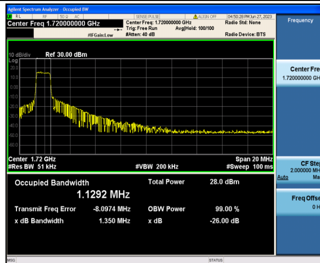
Band4-20MHz-16QAM-20050-6-0-Low-1.1292-1.350-PASS
