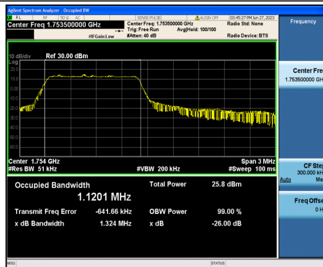
Band4-3MHz-QPSK-20385-6-0-Low-1.1201-1.324-PASS
