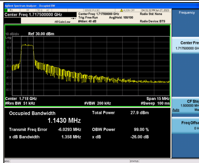
Band4-15MHz-QPSK-20025-6-0-Low-1.1430-1.358-PASS
