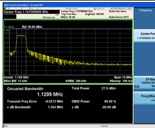
Band4-15MHz-16QAM-20325-6-0-Low-1.1299-1.354-PASS
