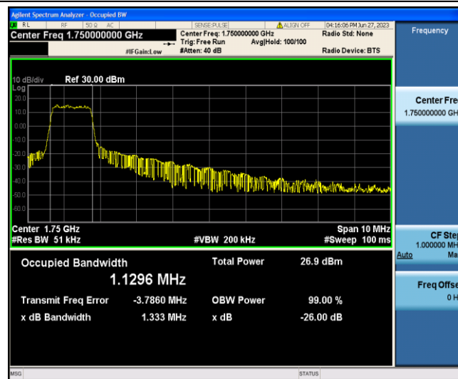
Band4-10MHz-QPSK-20350-6-0-Low-1.1296-1.333-PASS
