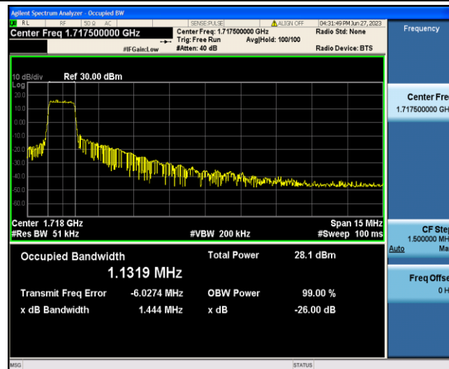
Band4-15MHz-16QAM-20025-6-0-Low-1.1319-1.444-PASS
