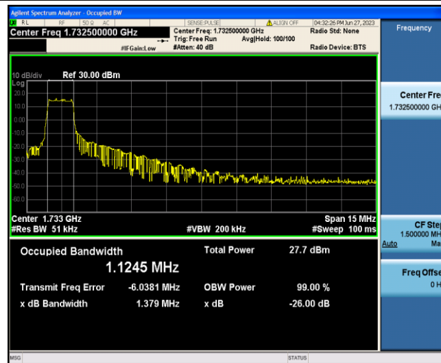
Band4-15MHz-16QAM-20175-6-0-Low-1.1245-1.379-PASS
