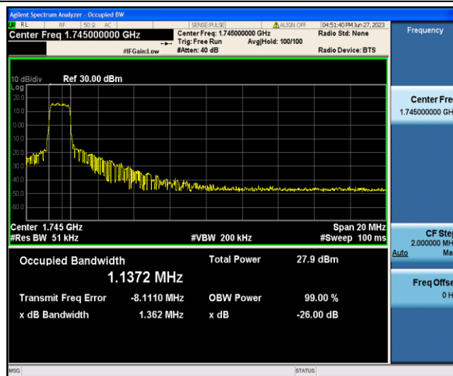
Band4-20MHz-16QAM-20300-6-0-Low-1.1372-1.362-PASS
