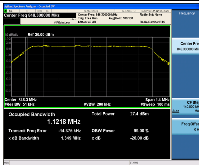
Band5-1.4MHz-QPSK-20643-6-0-Low-1.1218-1.349-PASS
