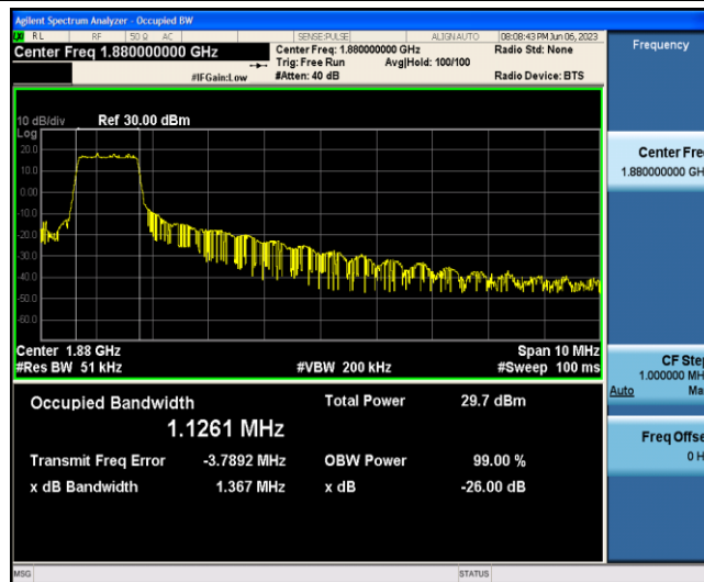
Band2-10MHz-16QAM-18900-6-0-Low-1.1261-1.367-PASS
