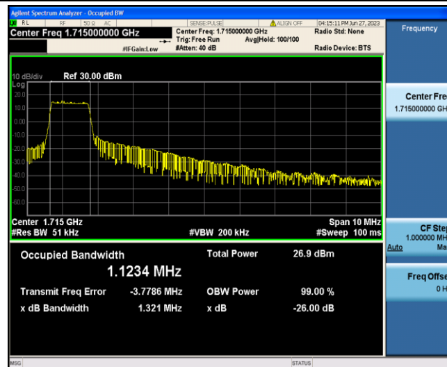
Band4-10MHz-16QAM-20000-6-0-Low-1.1234-1.321-PASS
