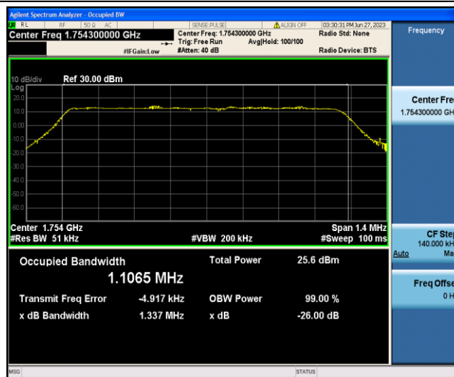
Band4-1.4MHz-16QAM-20393-6-0-Low-1.1065-1.337-PASS
