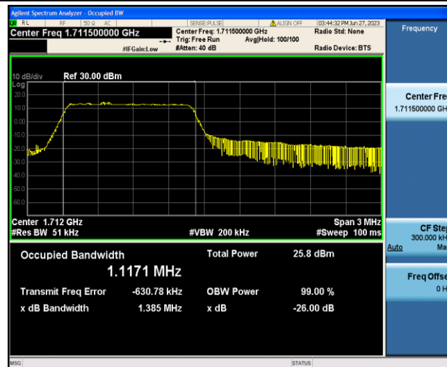
Band4-3MHz-16QAM-19965-6-0-Low-1.1171-1.385-PASS
