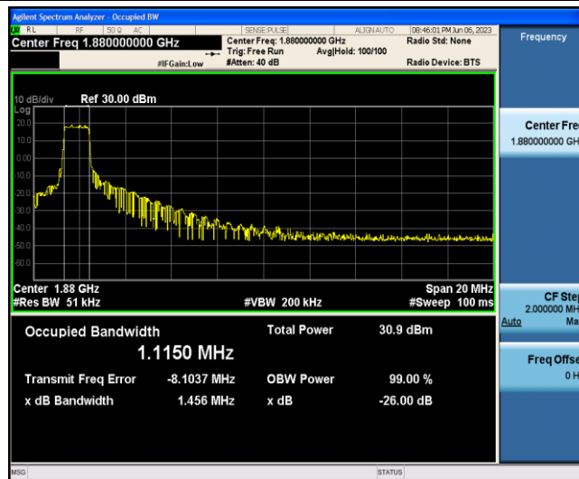
Band2-20MHz-QPSK-18900-6-0-Low-1.1150-1.456-PASS
