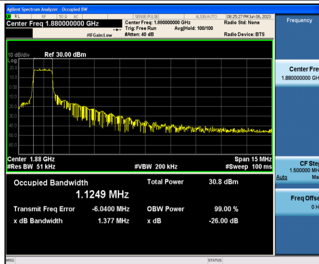
Band2-15MHz-16QAM-18900-6-0-Low-1.1249-1.377-PASS
