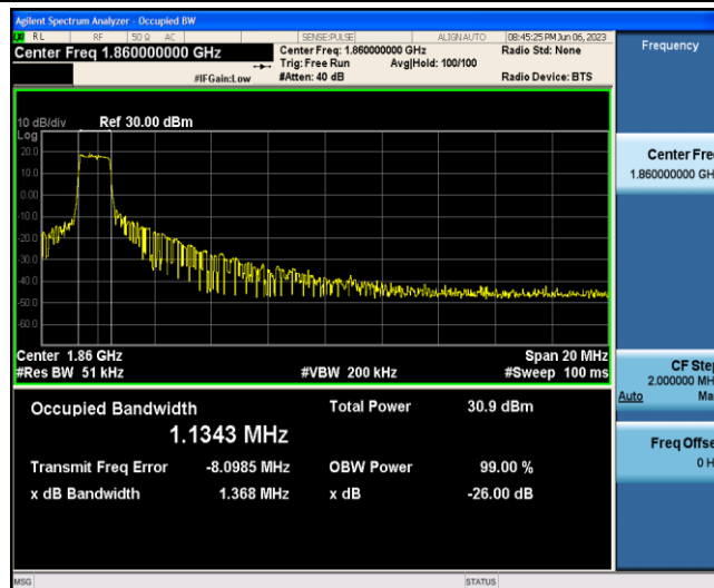
Band2-20MHz-QPSK-18700-6-0-Low-1.1343-1.368-PASS
