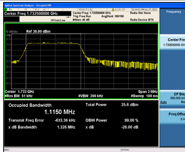
Band4-3MHz-QPSK-20175-6-0-Low-1.1150-1.326-PASS
