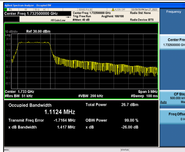
Band4-5MHz-QPSK-20175-6-0-Low-1.1124-1.417-PASS
