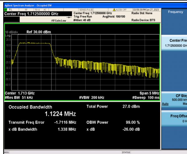
Band4-5MHz-16QAM-19975-6-0-Low-1.1224-1.338-PASS
