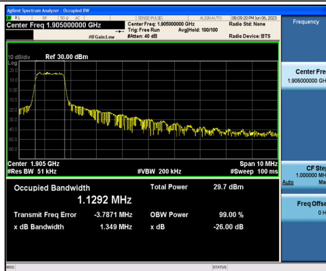
Band2-10MHz-16QAM-19150-6-0-Low-1.1292-1.349-PASS
