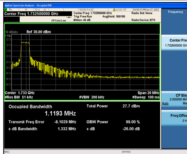
Band4-20MHz-QPSK-20175-6-0-Low-1.1193-1.332-PASS
