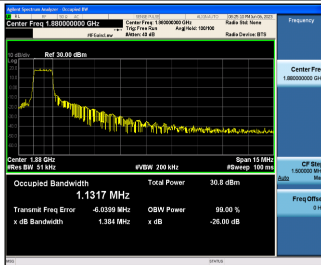
Band2-15MHz-QPSK-18900-6-0-Low-1.1317-1.384-PASS
