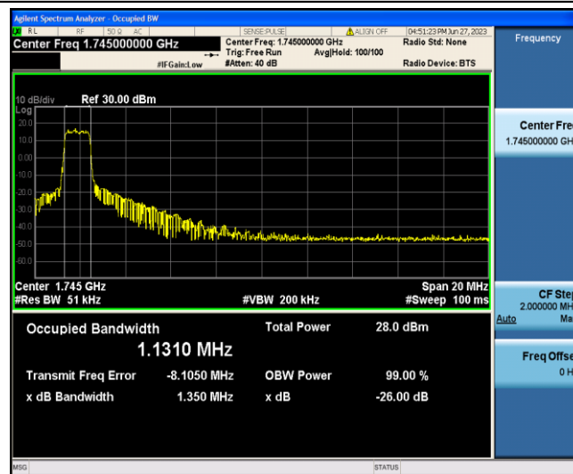
Band4-20MHz-QPSK-20300-6-0-Low-1.1310-1.350-PASS
