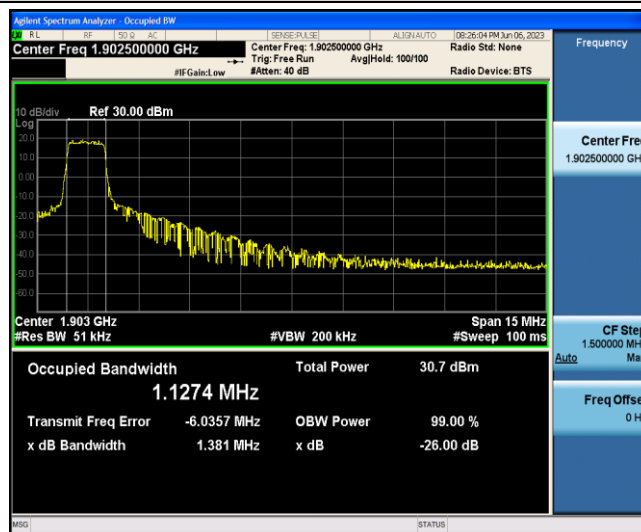
Band2-15MHz-16QAM-19125-6-0-Low-1.1274-1.381-PASS
