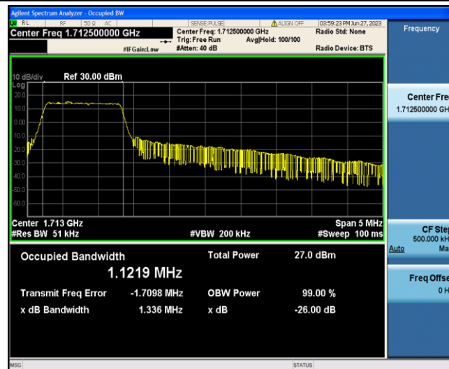
Band4-5MHz-QPSK-19975-6-0-Low-1.1219-1.336-PASS
