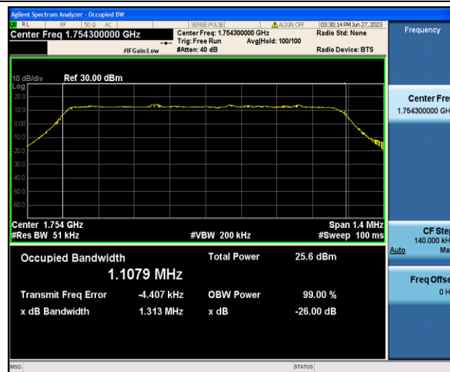
Band4-1.4MHz-QPSK-20393-6-0-Low-1.1079-1.313-PASS
