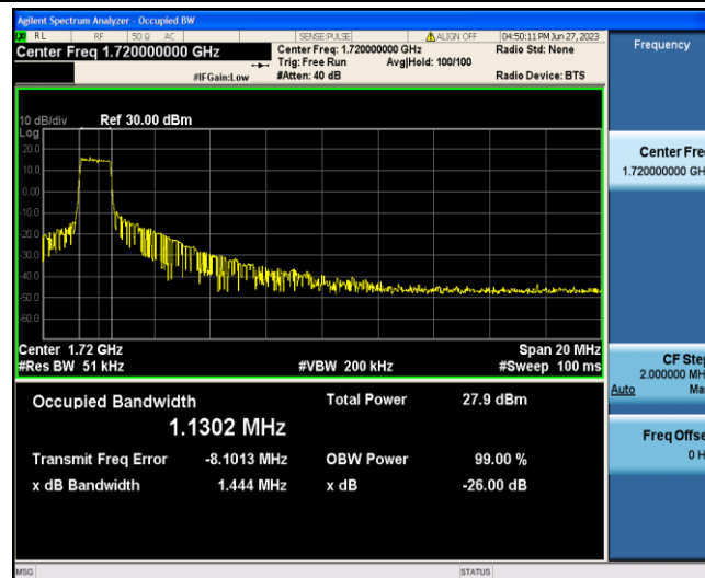
Band4-20MHz-QPSK-20050-6-0-Low-1.1302-1.444-PASS
