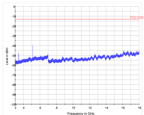
LTE Band 4 3MHz CH-Middle 3GHz~18GHz
