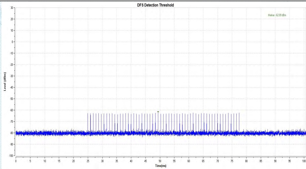
11A_5260_Type2
