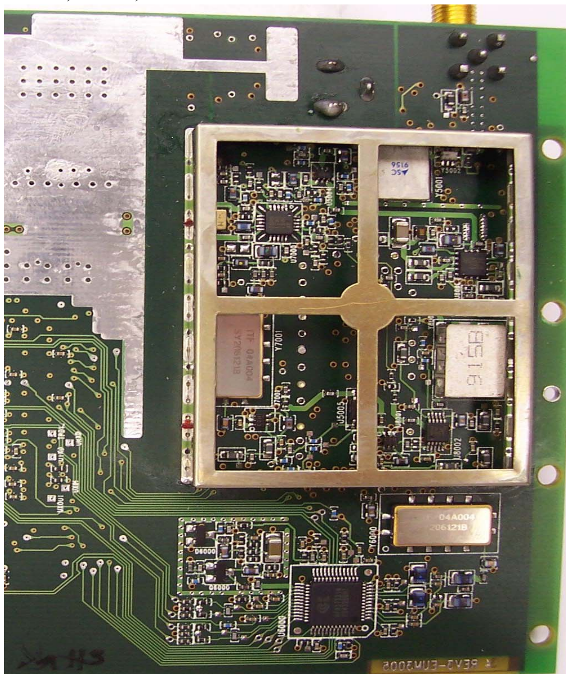
Bottom side, shield off, radio detail.
