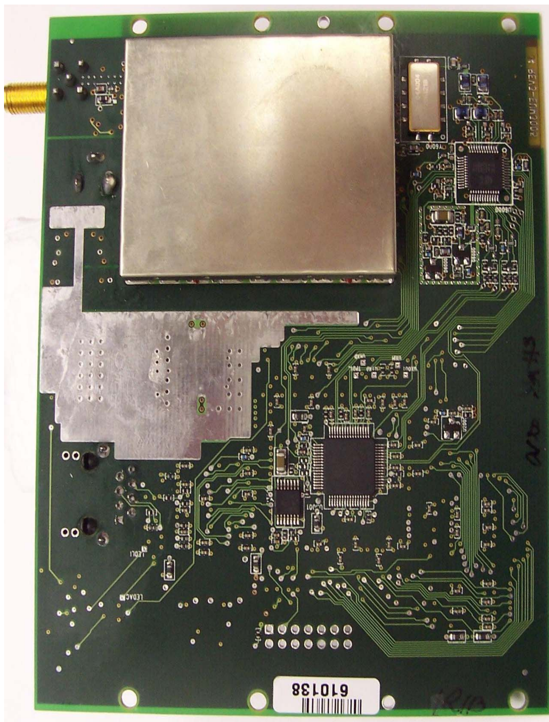
Bottom side with shield on
