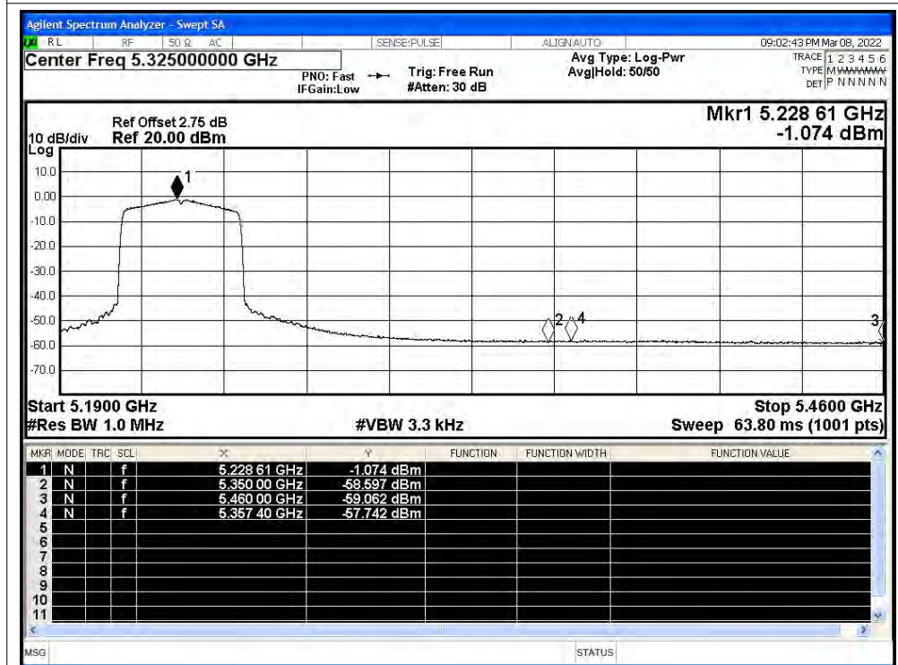
Restrict Band NVNT ax40 5230MHz Ant0+Ant1 Average
