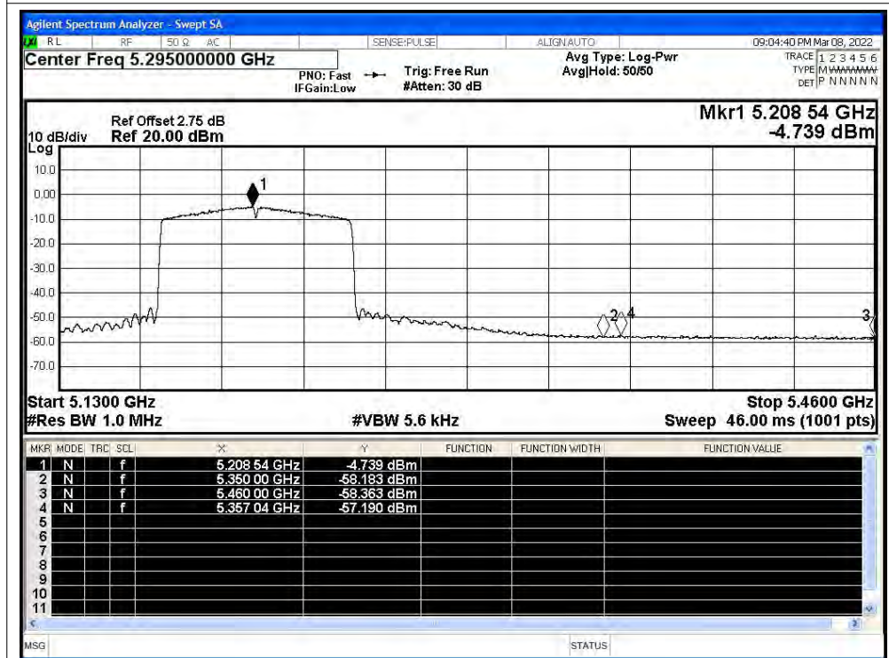
Restrict Band NVNT ac80 5210MHz Ant0+Ant1 Average
