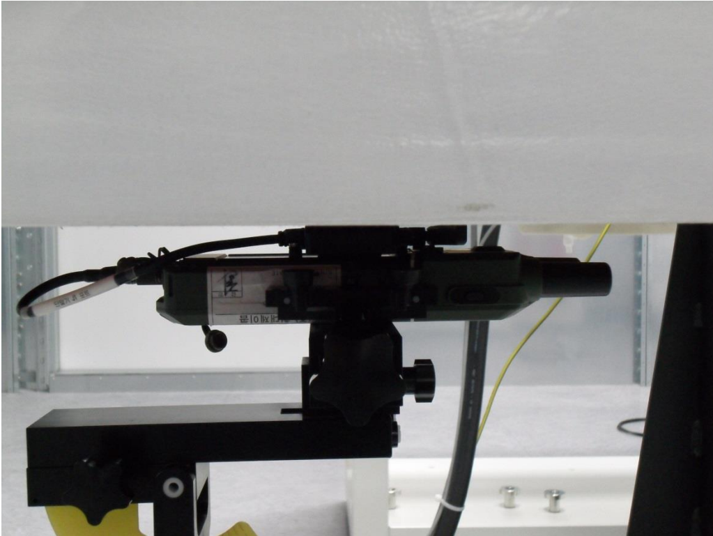
Rear with External Antenna _0 degree (0.0mm)
