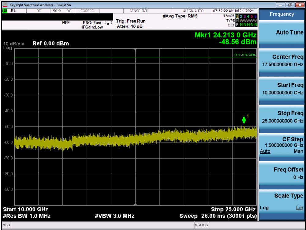
Plot 7-90. Conducted Spurious Plot (Bluetooth (LE), 1Mbps – Ch. 37) – Ant1
