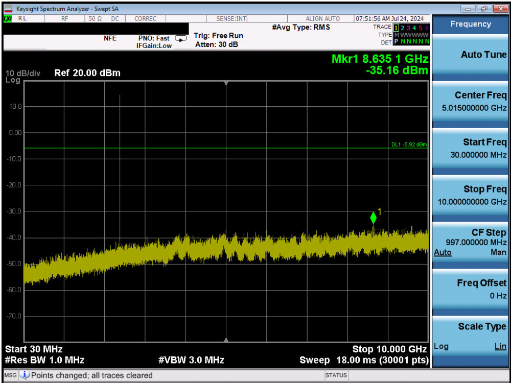
Plot 7-89. Conducted Spurious Plot (Bluetooth (LE), 1Mbps – Ch. 37) – Ant1
