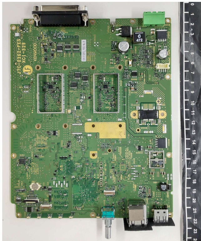
MAIN Unit without shield case
