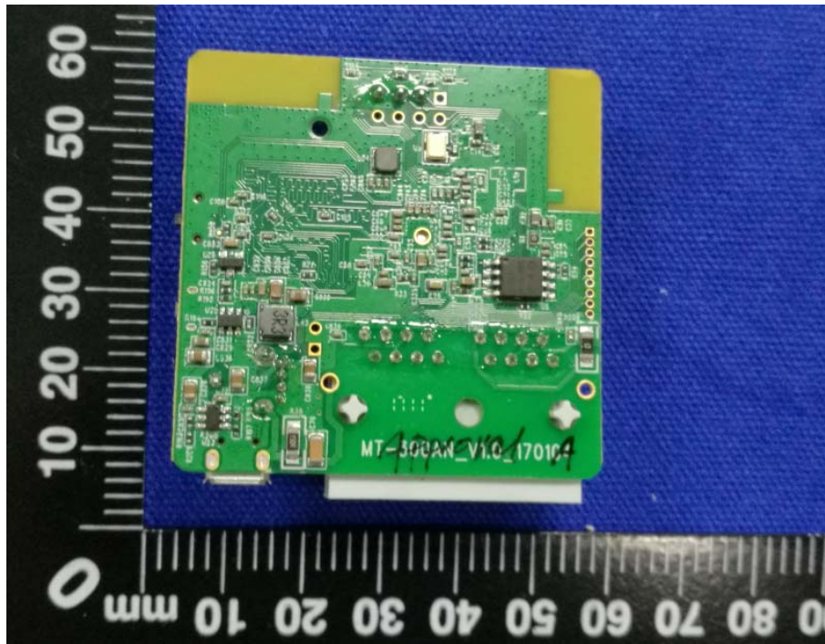
EUT –Wi-fi chip View
