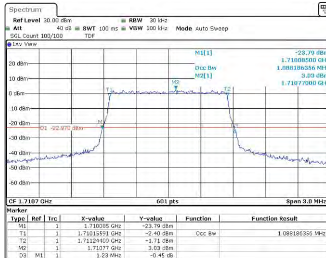
Band66-1.4MHz-16QAM-132322-6RB#0
