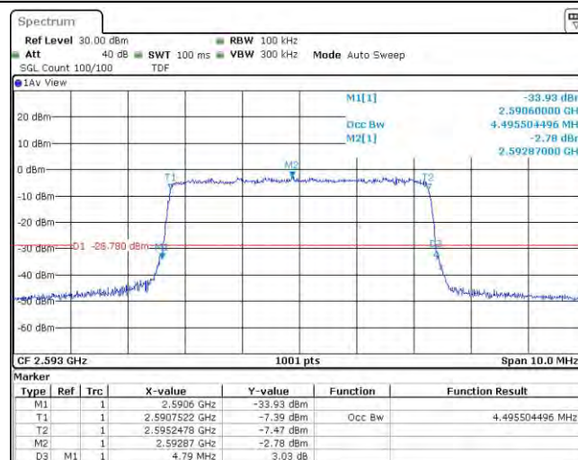
Band41-5MHz-16QAM-41565-25RB#0
