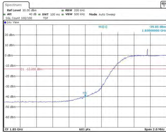
Band2-10MHz-QPSK-18650-1RB#49
