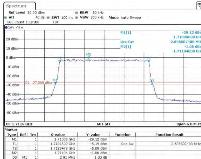
Band66-3MHz-16QAM-132322-15RB#0
