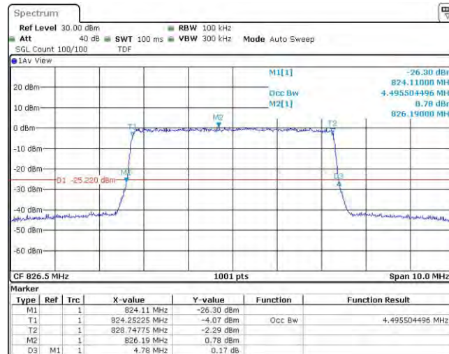
Band5-5MHz-16QAM-20525-25RB#0
