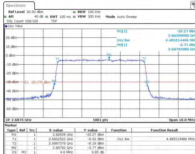
Band41-5MHz-16QAM-39675-25RB#0
