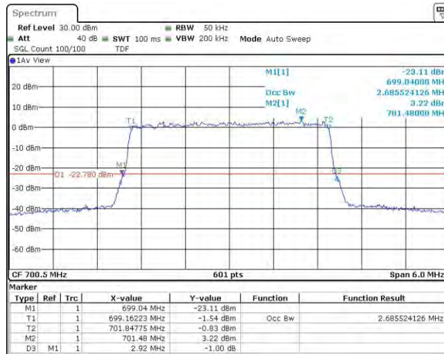
Band12-3MHz-16QAM-23095-15RB#0
