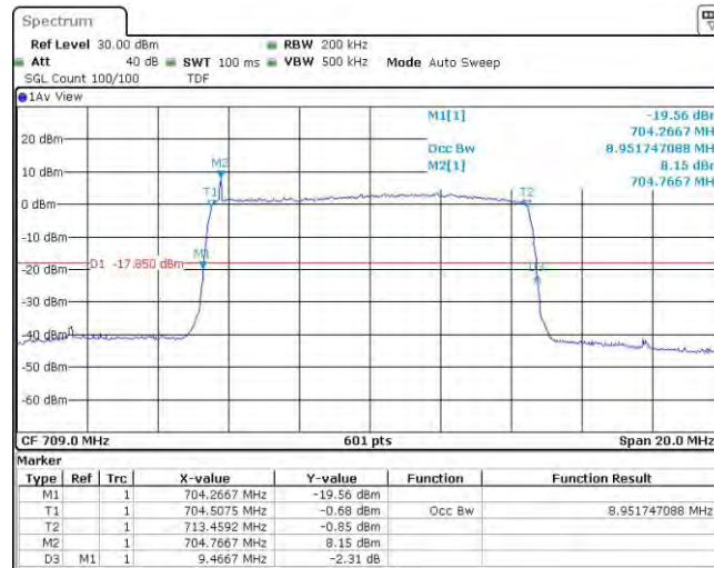
Band17-10MHz-QPSK-23790-50RB#0
