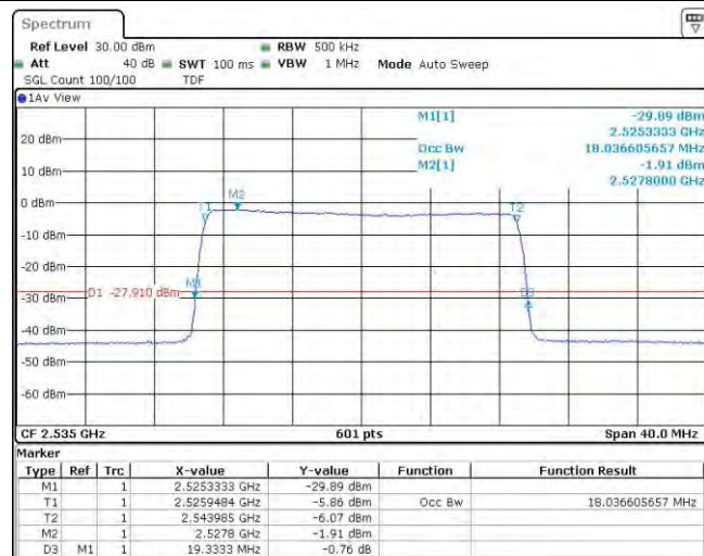
Band7-20MHz-16QAM-21350-100RB#0
