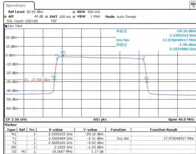
Band7-20MHz-16QAM-20850-100RB#0
