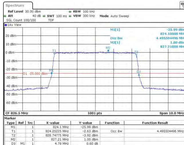
Band5-5MHz-QPSK-20525-25RB#0
