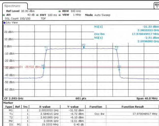
Band41-20MHz-16QAM-41490-100RB#0
