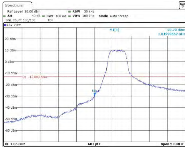
Band2-1.4MHz-QPSK-18607-1RB#5
