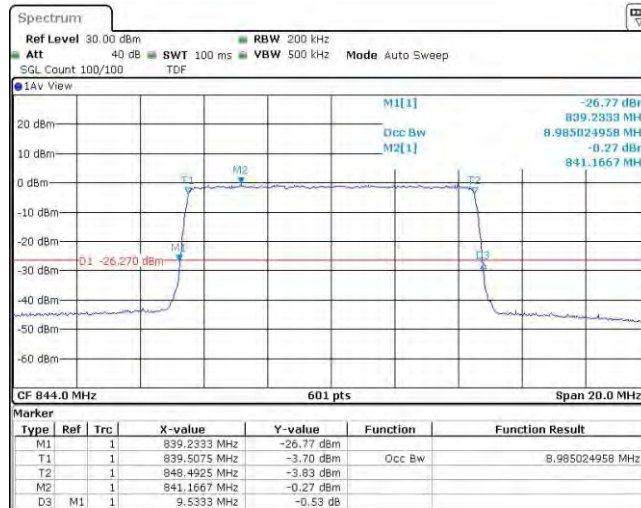
Band5-10MHz-16QAM-20450-50RB#0
