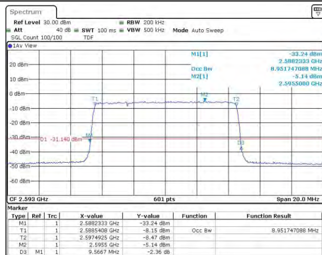
Band41-10MHz-16QAM-41540-50RB#0
