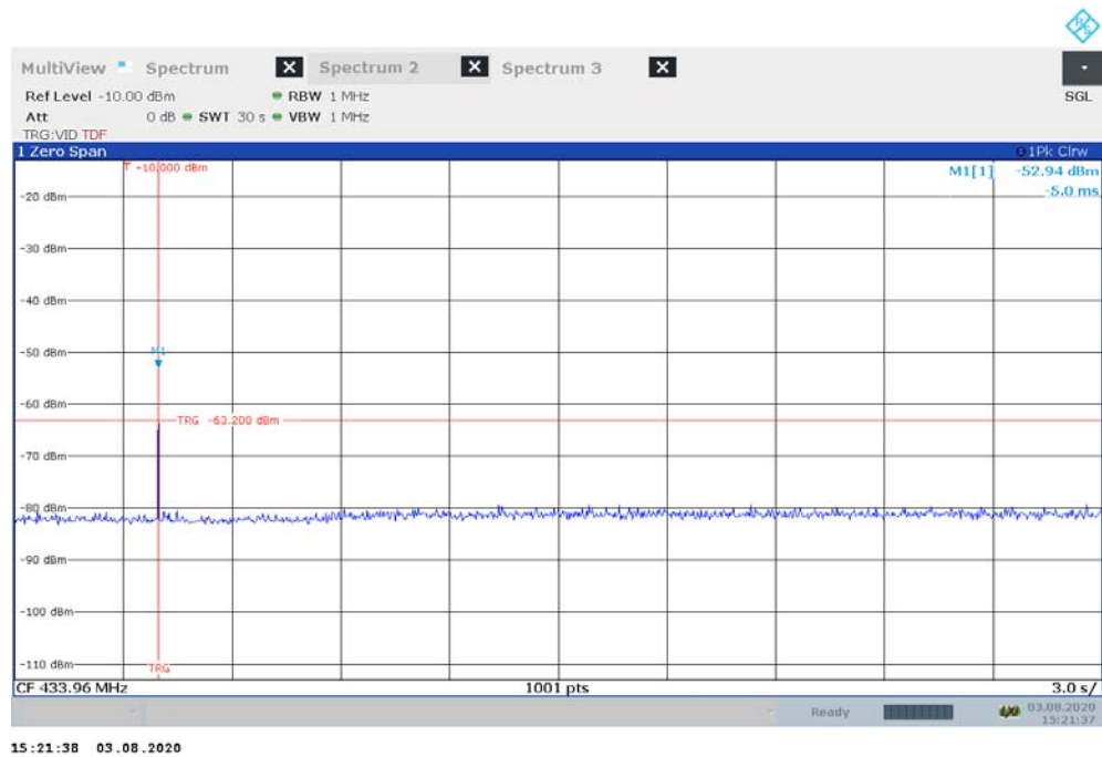
Figure 2. Plot of the Transmission Time (Operated from DC 12 V)
