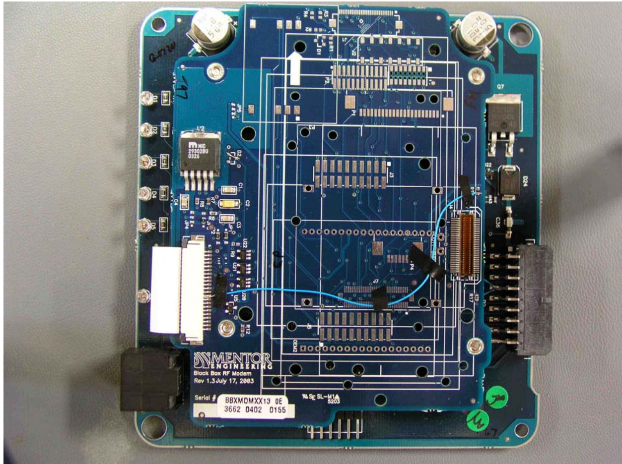
Top Assembly, no modem
