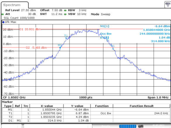
GSM_Low 0.244MHz
