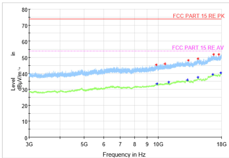
Fig.25 Radiated Spurious Emission (GFSK, Ch39, 3 GHz ~18 GHz), LE 1M
