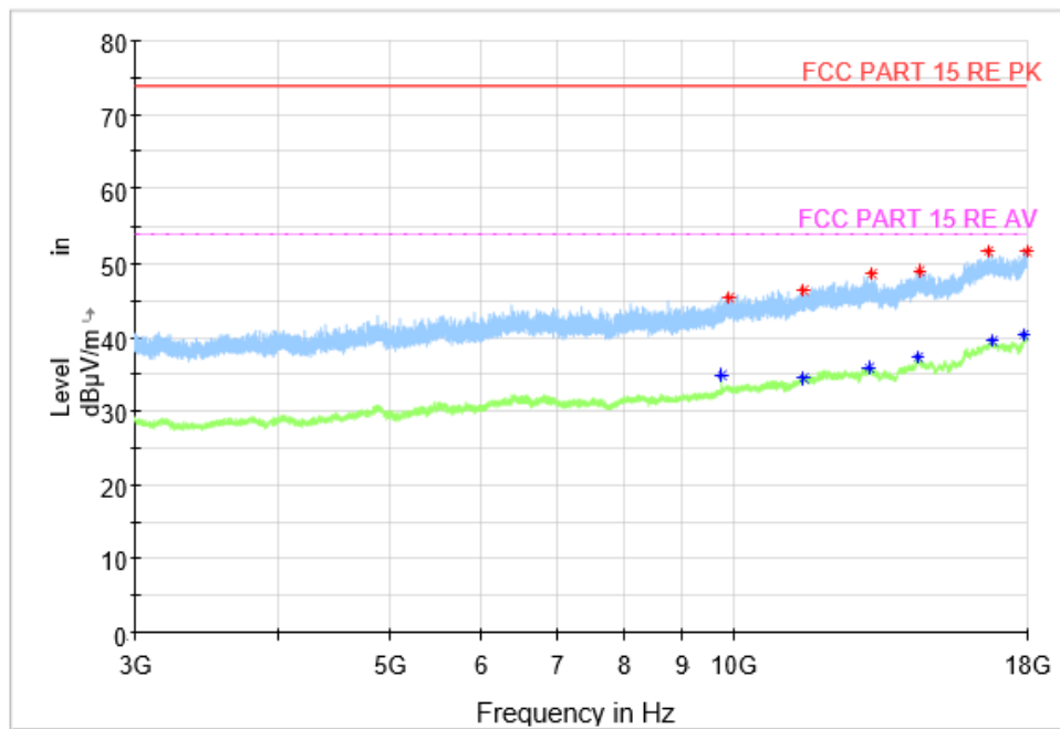
Fig.23 Radiated Spurious Emission (GFSK, Ch19, 3 GHz ~18 GHz), LE 1M
