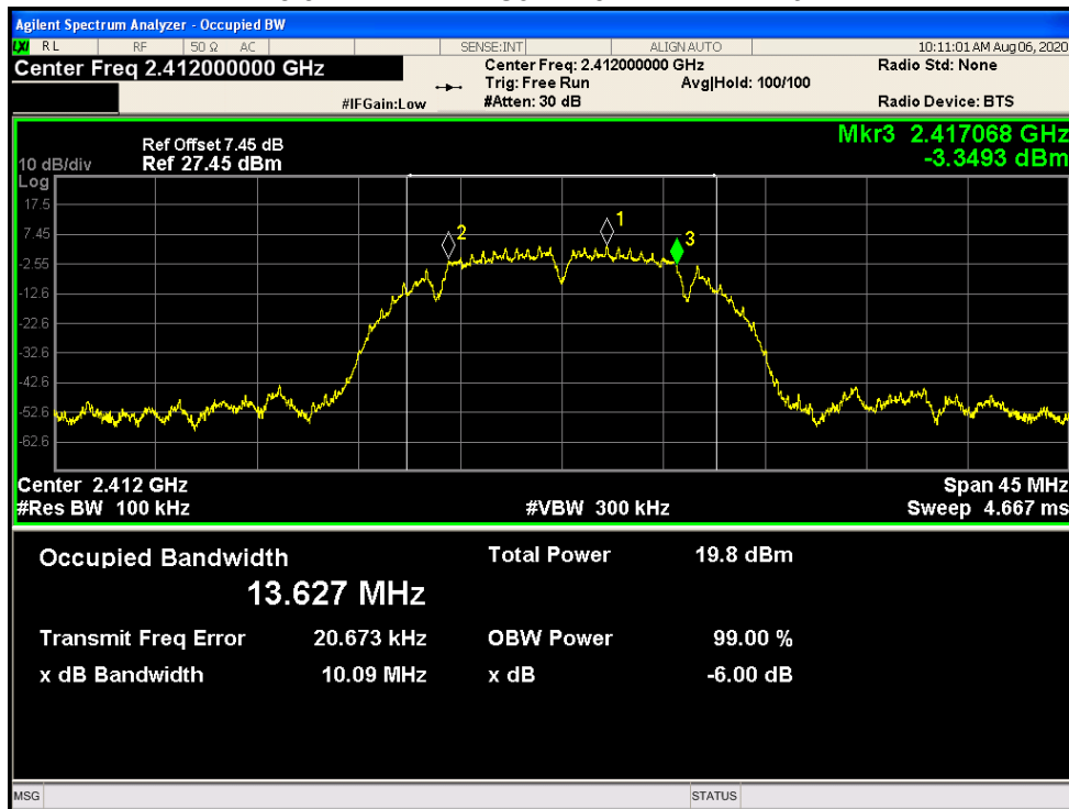
-6 dB BW NVHT 802.11b 2412MHz Ant 1
