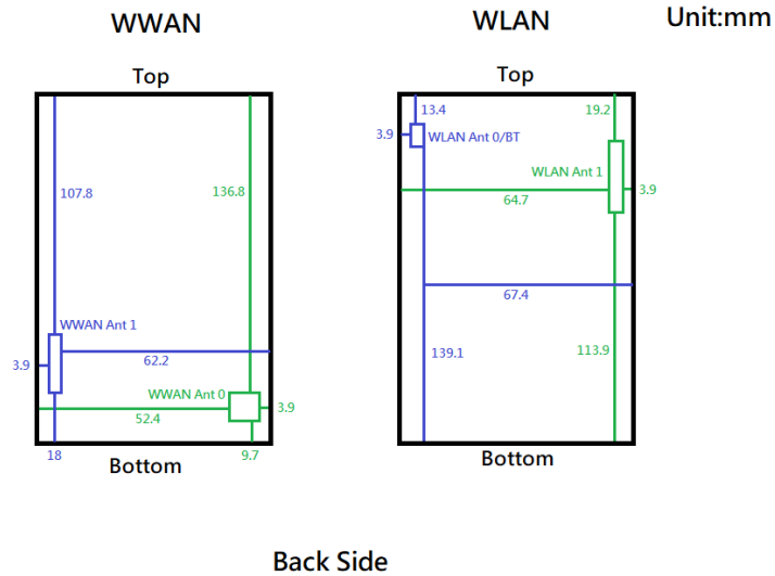
Fig.23 Antenna position of EUT
