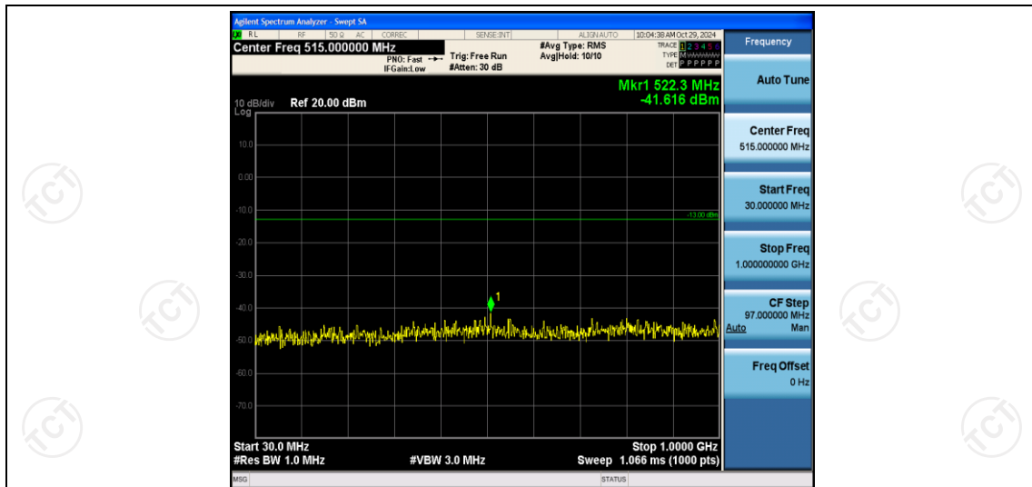
Band2-1.4MHz-QPSK-18607-1RB#0-Range1:30~1000MHz
