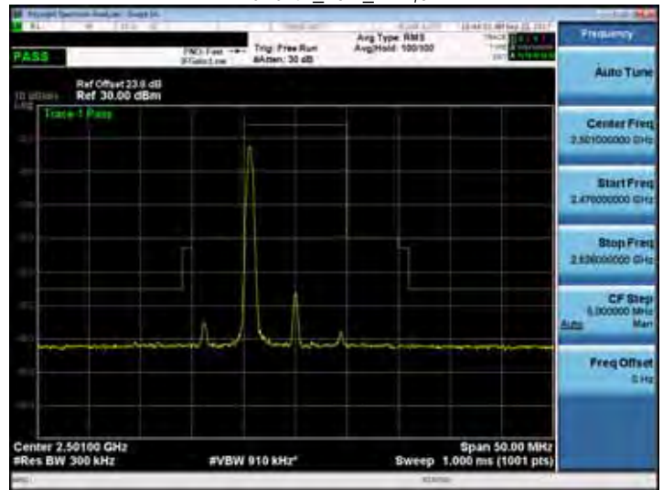
Band 41_10M_RB1,49
