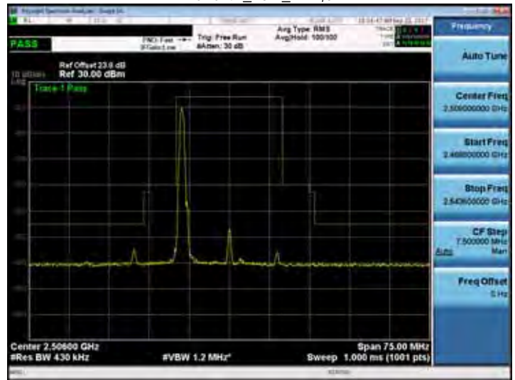
Band 41_20M_RB1,99
