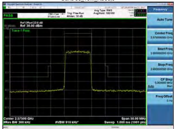
Band 38_10M_RB50,0
