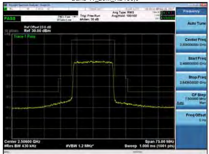
Band 41_20M_RB100,0
