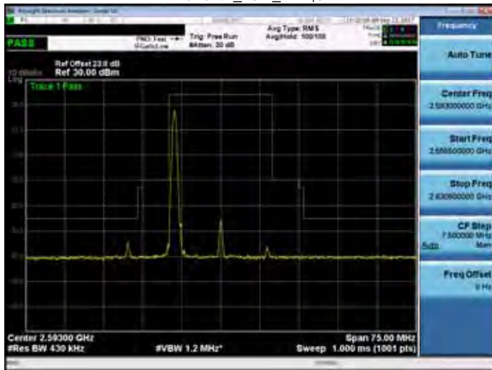
Band 41_20M_RB1,99
