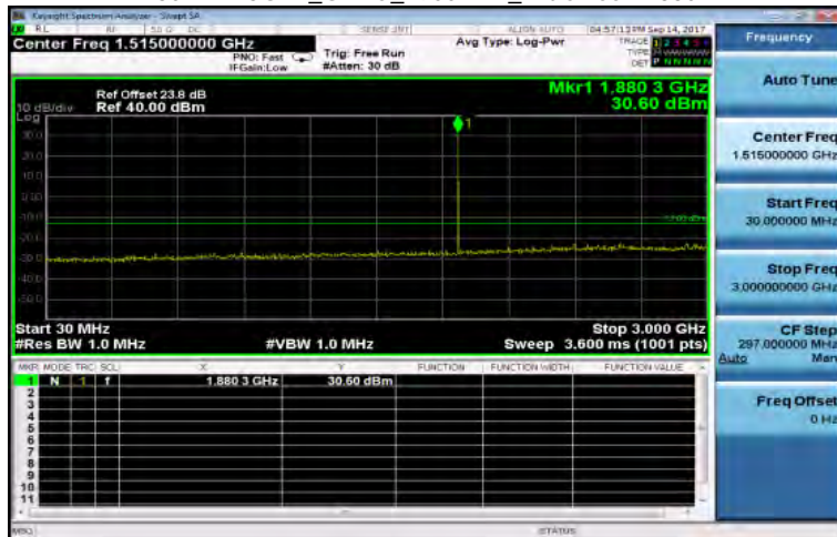
30MHz~3GHz_GPRS_1900MHz_MidCH661-1880
