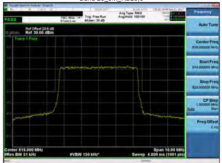
Band 26_5M_RB25,0
