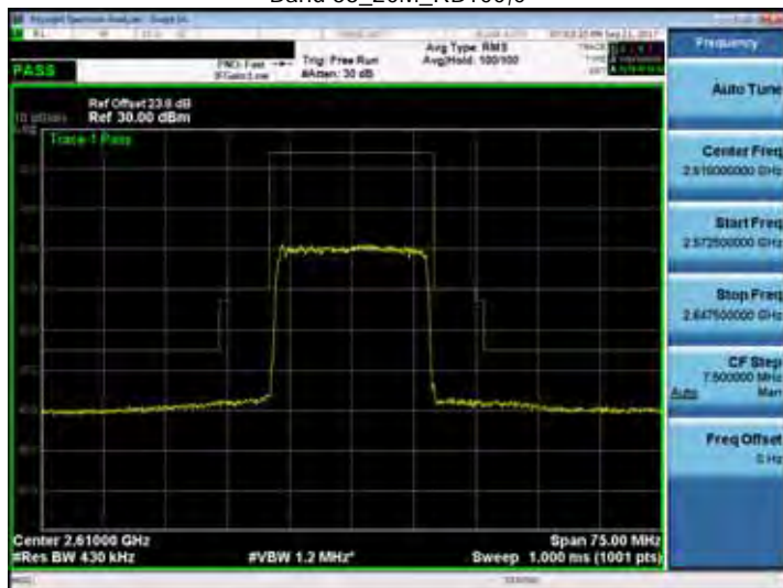
Band 38_20M_RB100,0
