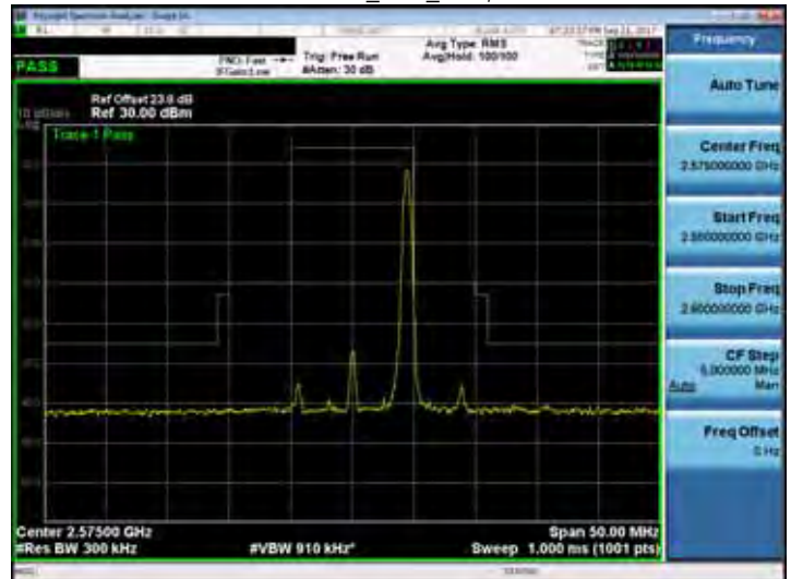
Band 38_10M_RB50,0
