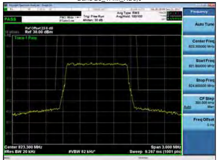
Band 26_1.4M_RB6,0
