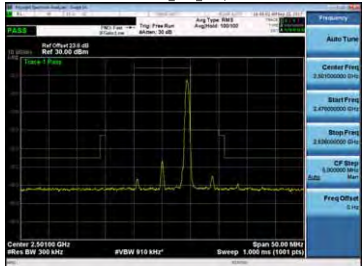
Band 41_10M_RB50,0
