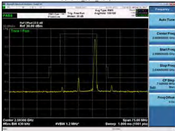
Band 41_20M_RB100,0
