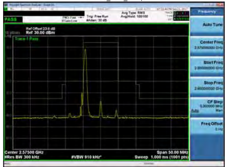
Band 38_10M_RB1,49
