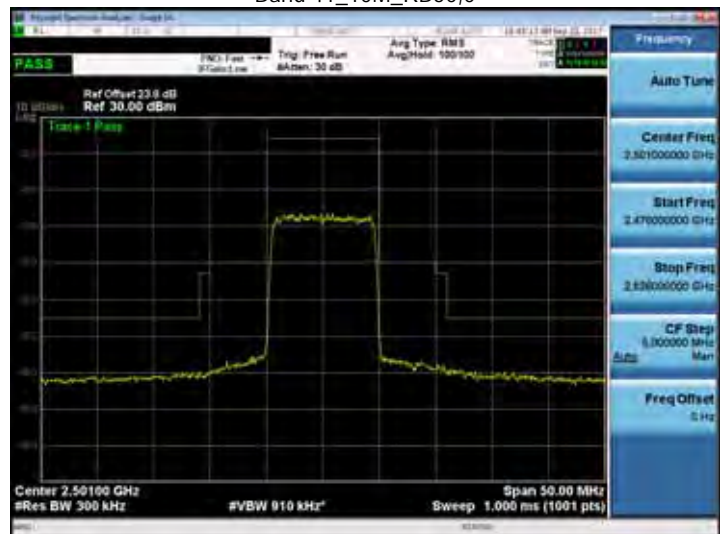
Band 41_10M_RB50,0
