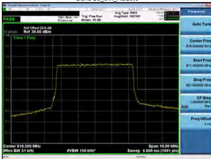
Band 26_5M_RB25,0
