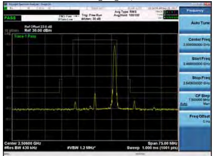
Band 41_20M_RB100,0
