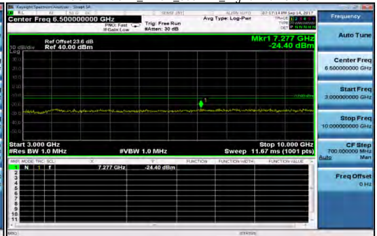
3GHz~10GHz_EDGE_850MHz_HighCH251-848.8
