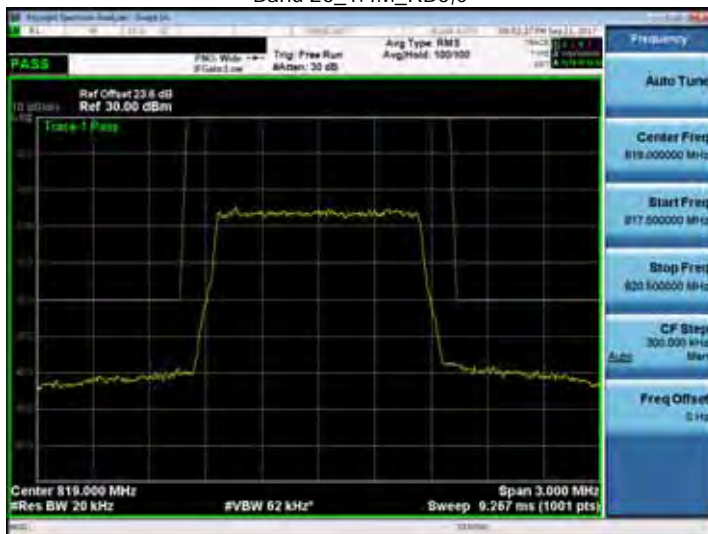
Band 26_1.4M_RB6,0
