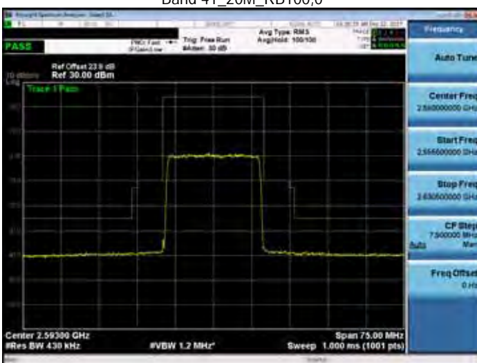
Band 41_20M_RB100,0
