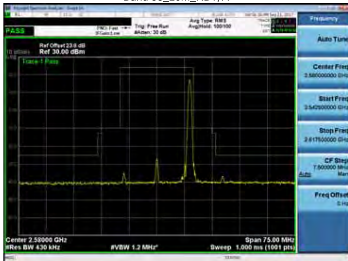
Band 38_20M_RB100,0
