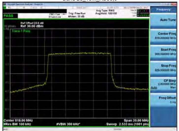
Band 26_10M_RB50,0
