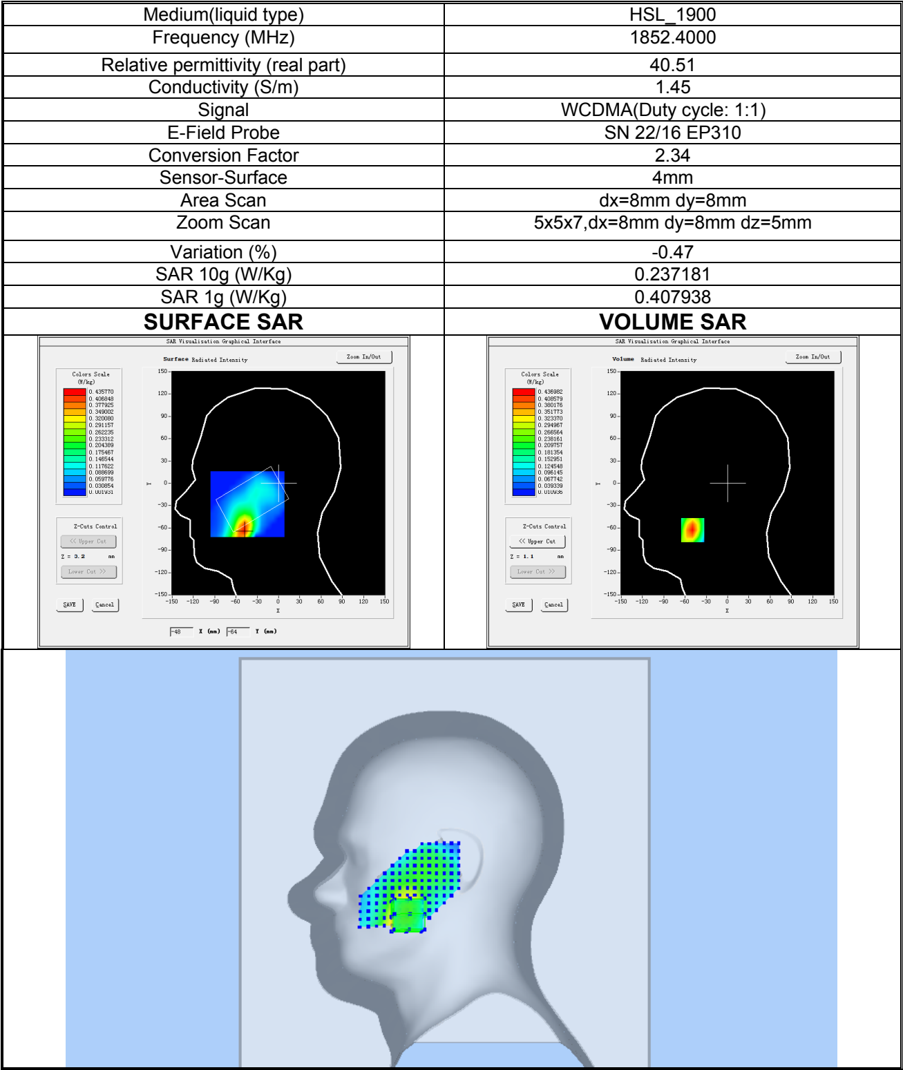
Plot 7: WCDMA BAND II , Low channel (Right Head Cheek) Product Description: Smartphone Test Date: 2022-04-06
