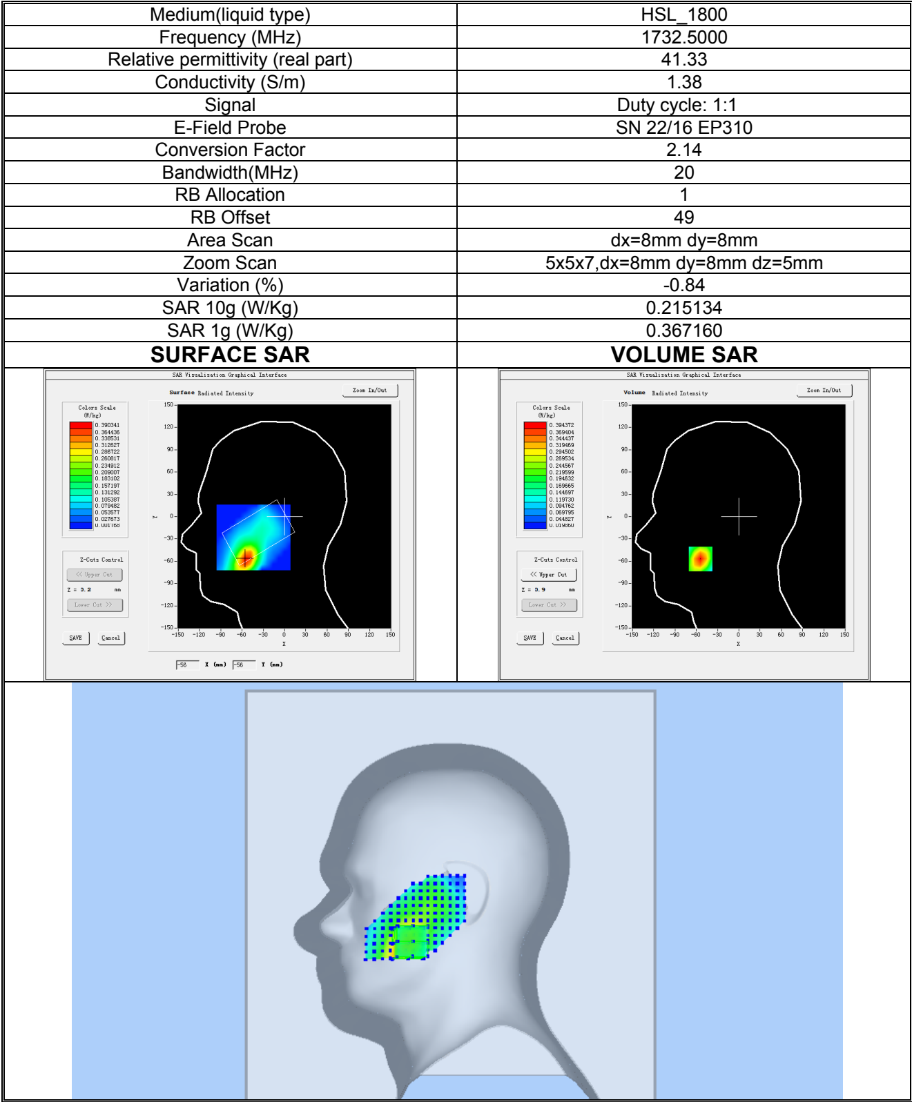
Plot 9:LTE BAND 4, Middle channel (Right Head Cheek) Product Description:Smartphone Test Date: 2022-03-26
