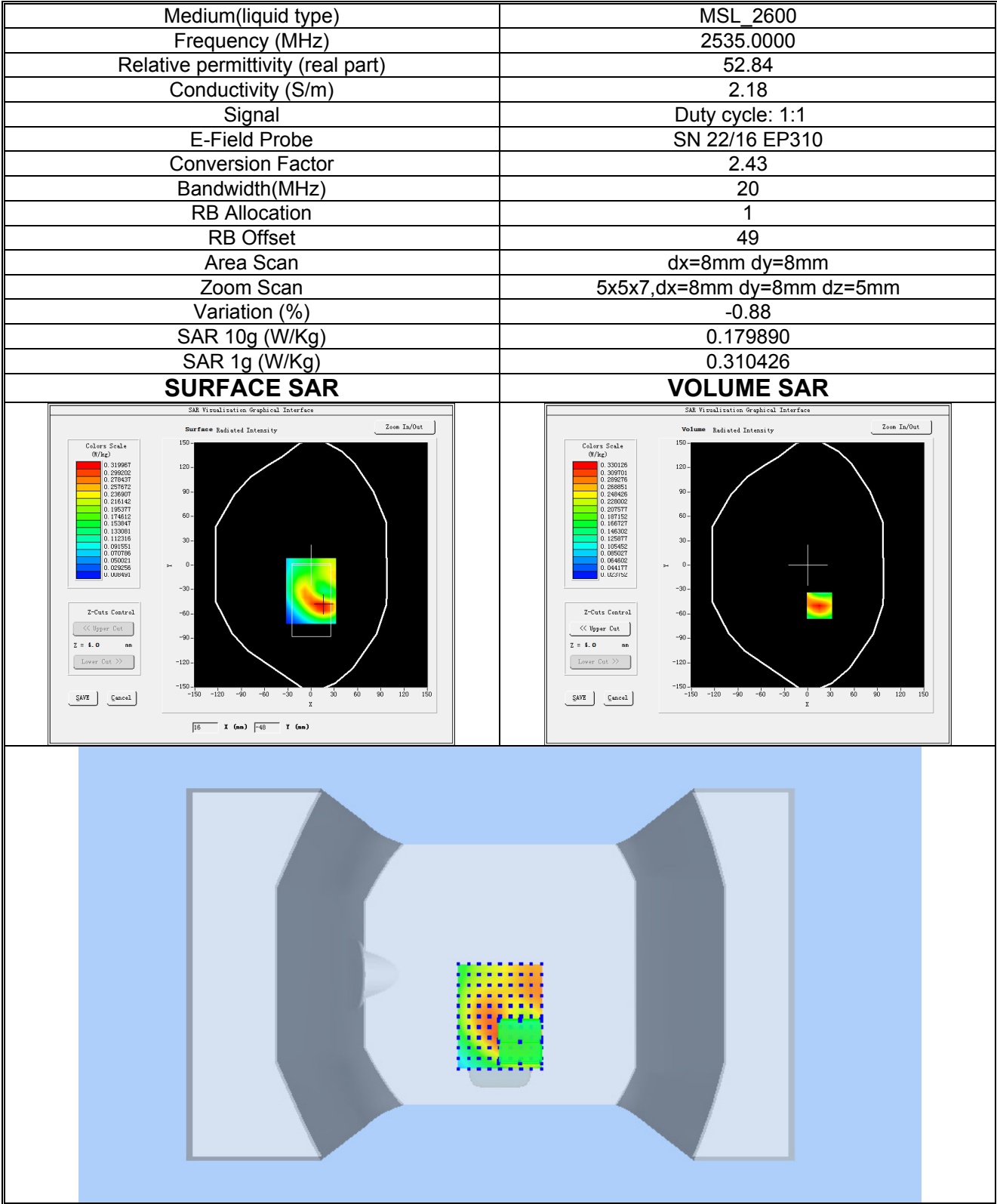
Plot 12:LTE BAND 7, Mid channel (Body-worn/ Hotspot, Back Side) Product Description: Smartphone Test Date: 2022-04-14
