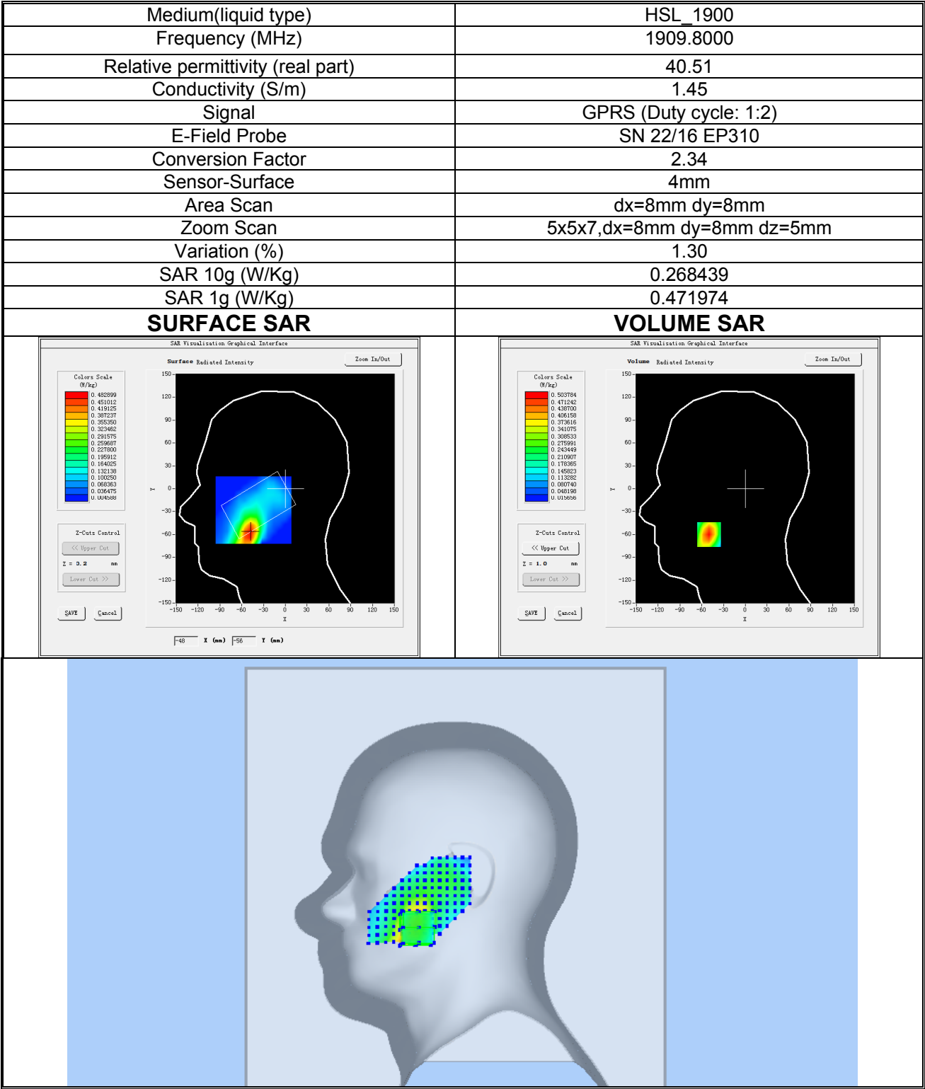
Plot 3: GPRS1900, high channel (Right Head Cheek) Product Description: Smartphone Test Date: 2022-04-06
