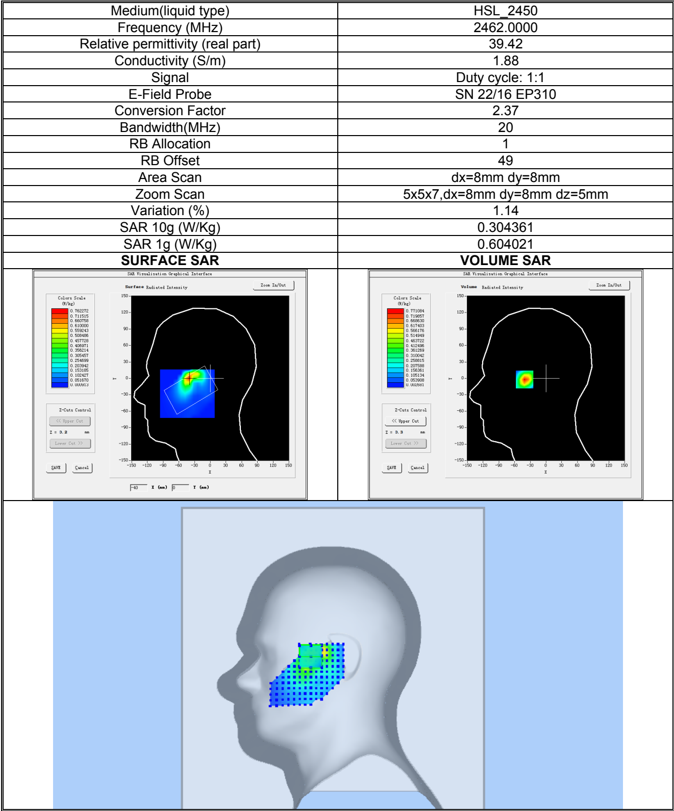
Plot 13:802.11b, High channel (Right Head Cheek) Product Description: Smartphone Test Date: 2022-04-11
