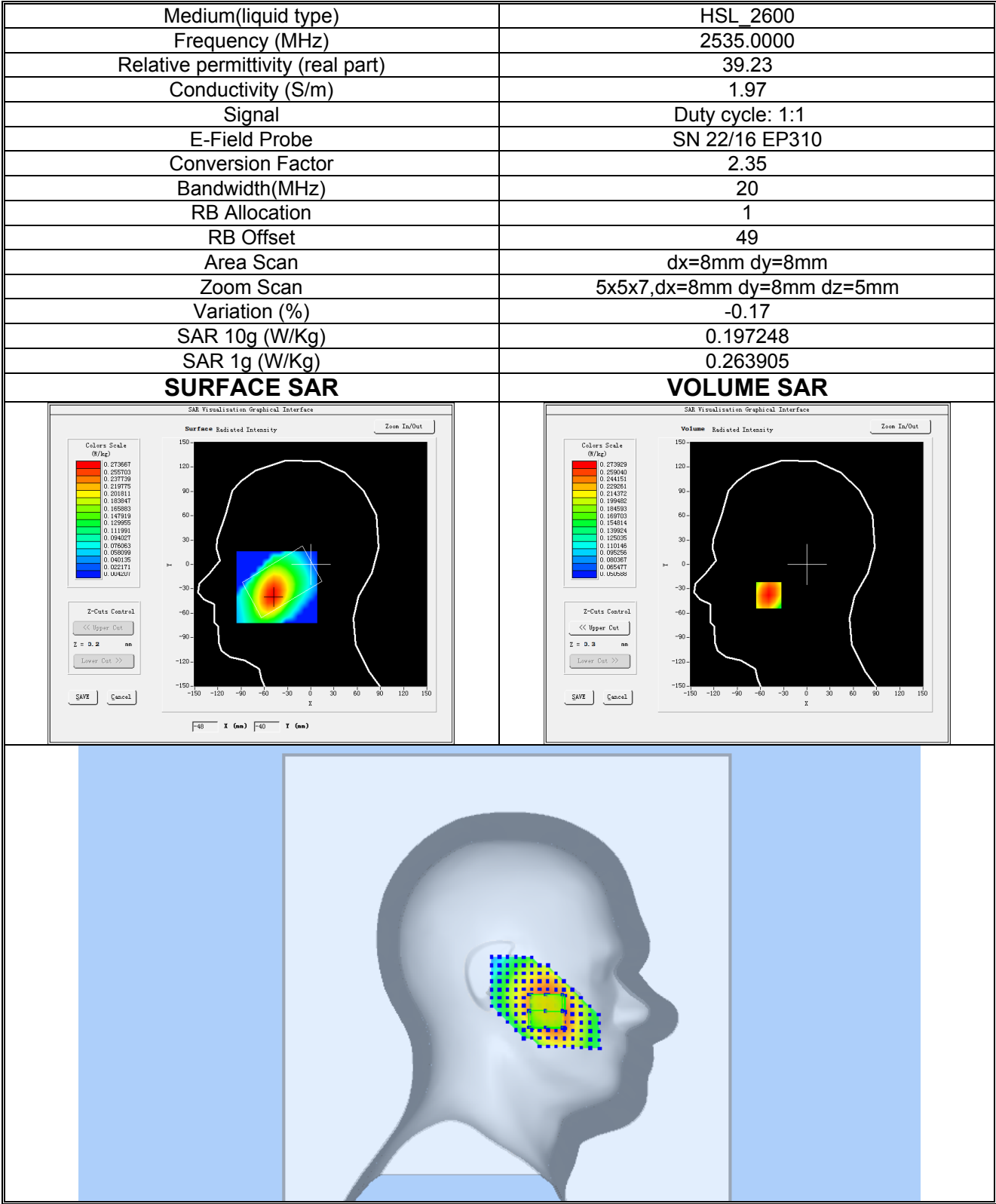
Plot 11:LTE BAND 7, Mid channel (Left Head Cheek) Product Description: Smartphone Test Date: 2022-04-14
