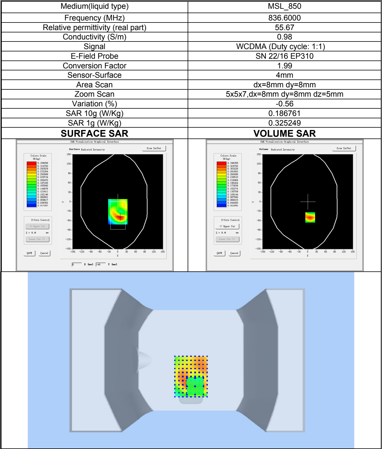
Plot 6: WCDMA BAND V, Mid channel (Body-worn /Hotspot, Back side) Product Description: Smartphone Test Date: 2022-03-21
