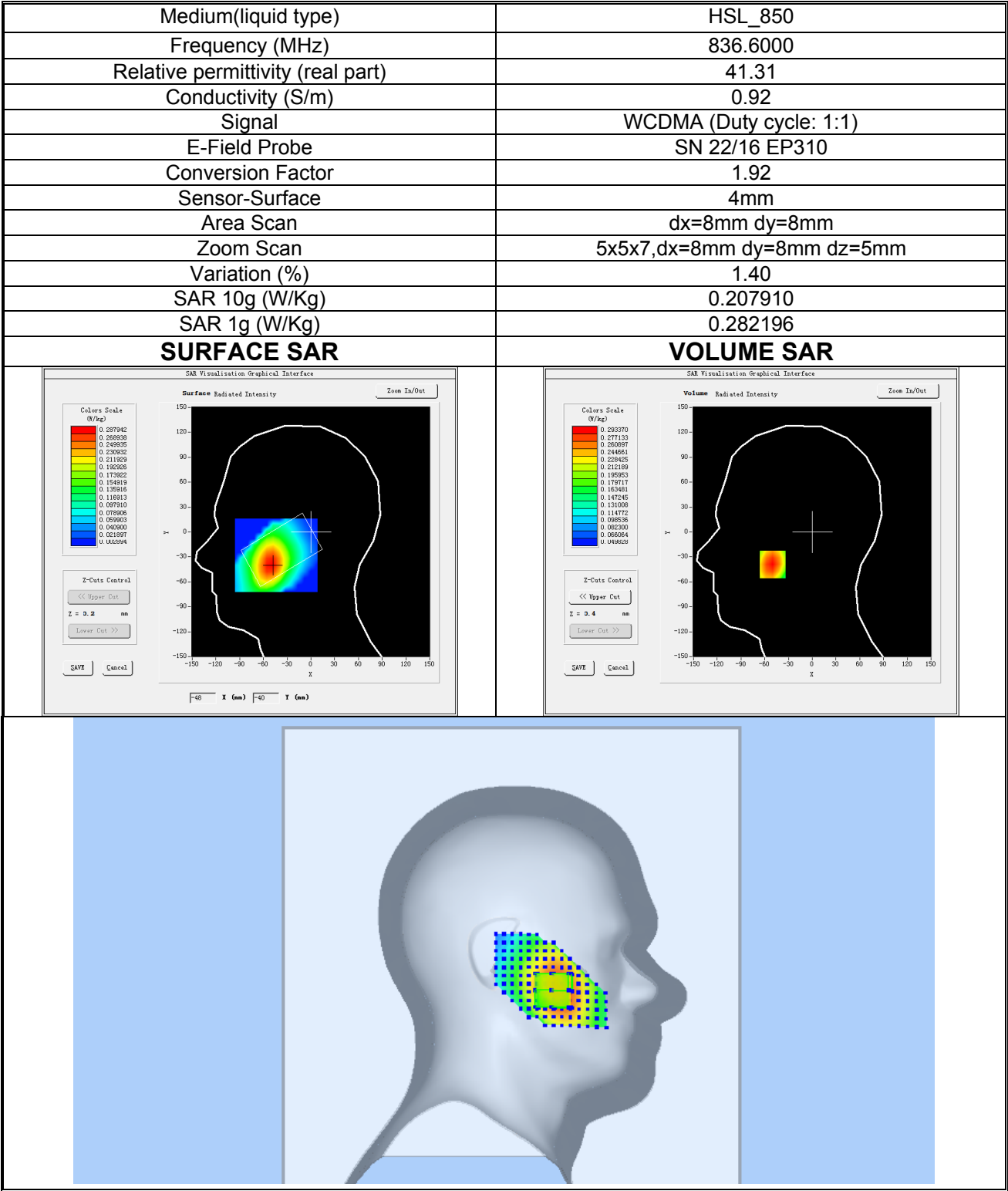
Plot 5: WCDMA BAND V, Mid channel (Left Head Cheek) Product Description: Smartphone Test Date: 2022-03-21
