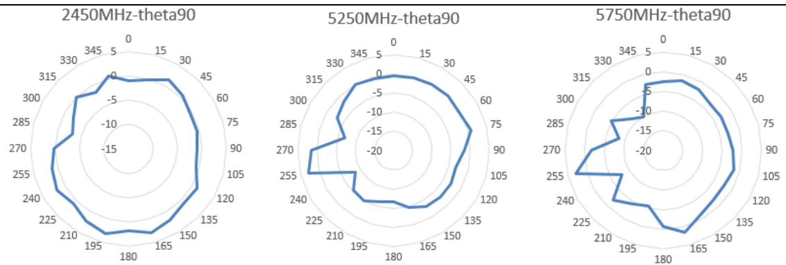
Ant3
