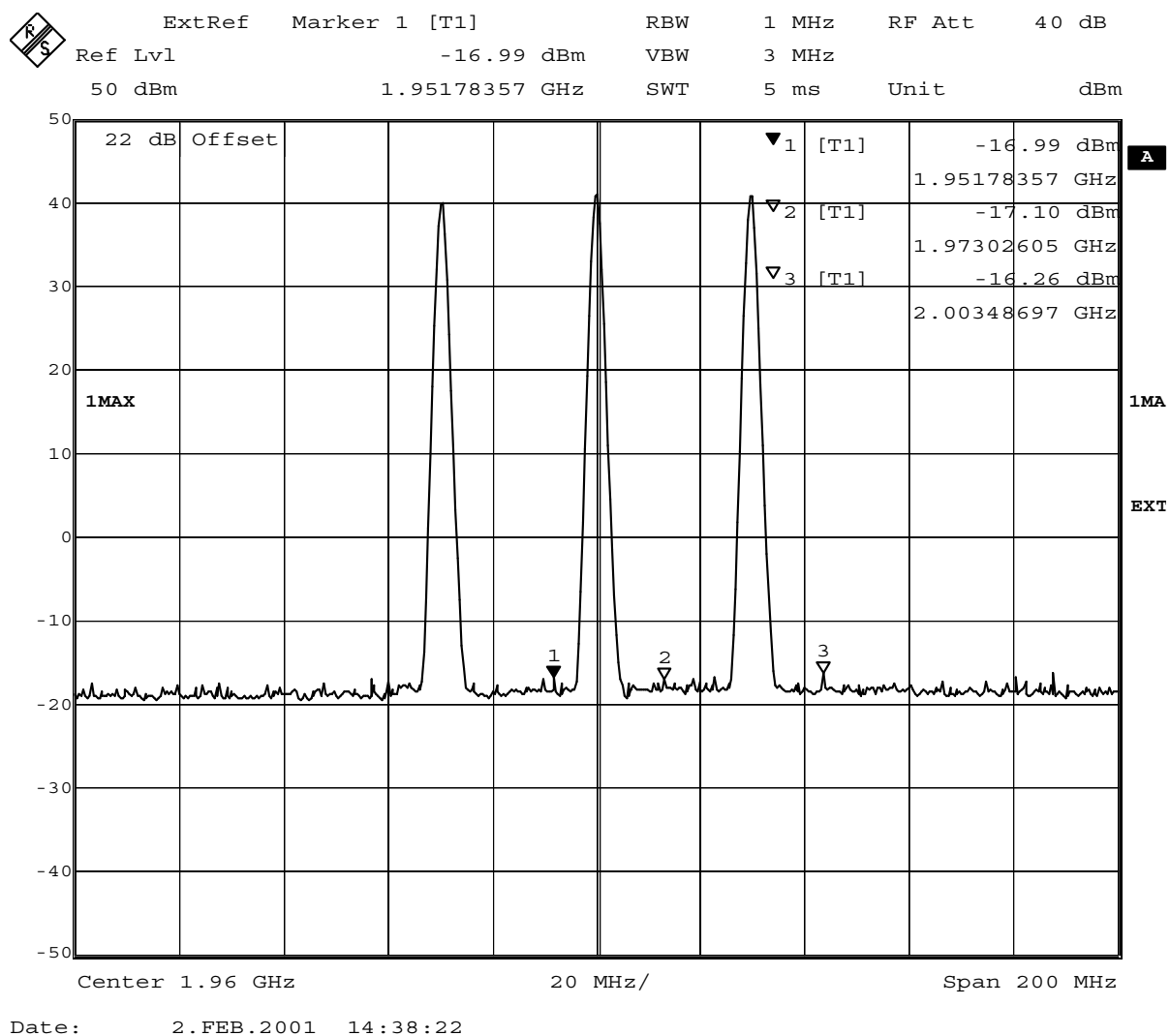
Fig. 41 – Slow frequency hopping – RBW = 1 MHz
