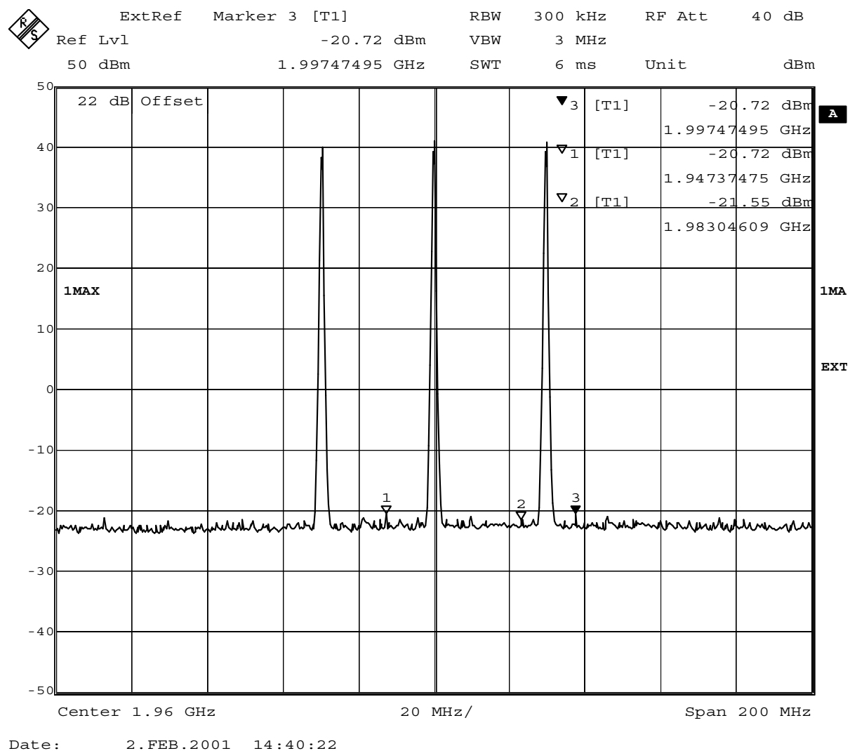
Fig. 42 – Slow frequency hopping – RBW = 300 kHz
