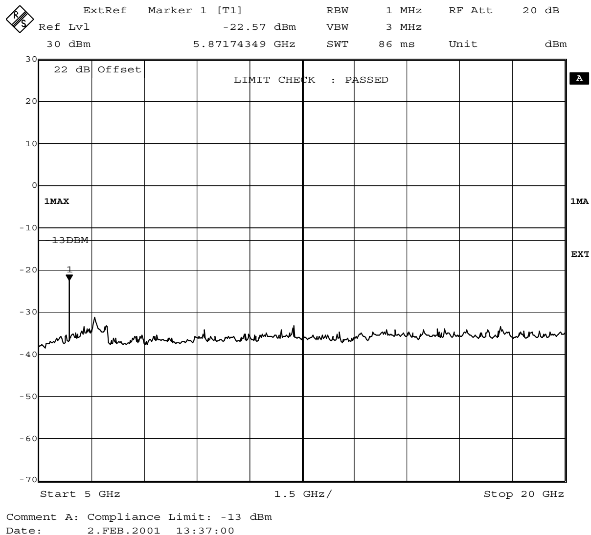
Fig. 22 – Spurious emissions in the frequency range 5000 MHz – 20000 MHz.
