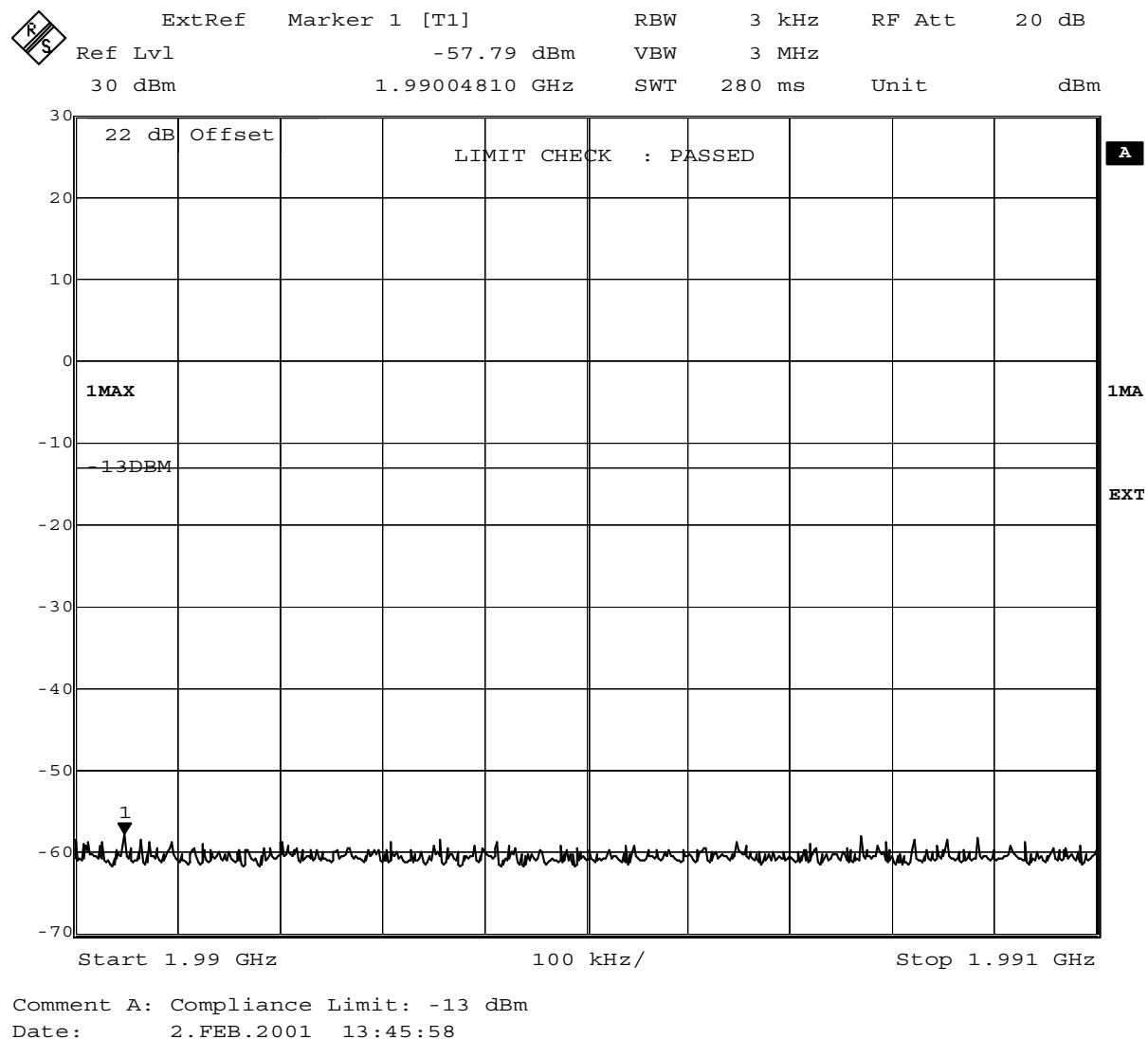
Fig. 12 – Spurious emissions in the frequency range 1990 MHz – 1991 MHz.
