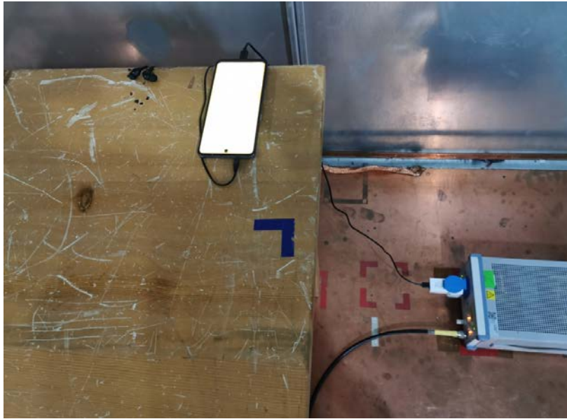
Conducted Emissions Test Setup (with charger)
