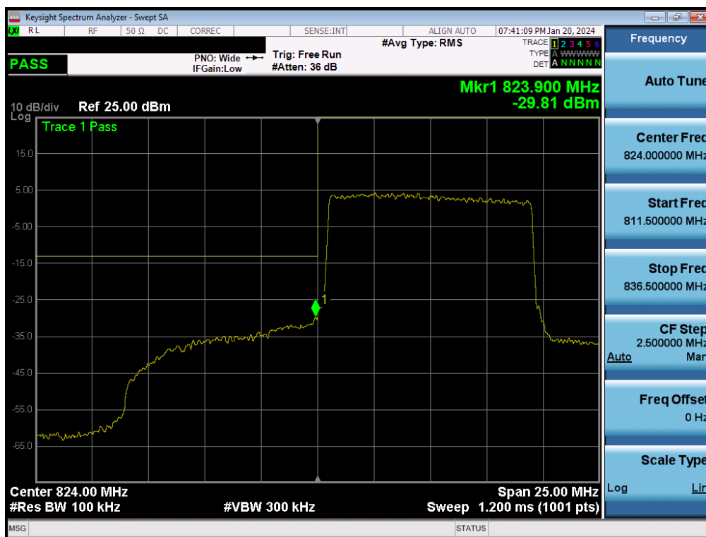
Plot 7-18. Lower Band Edge Plot (LTE Band 5 - 10MHz QPSK – Full RB)
