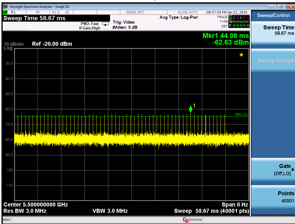
Radar Signal 1
