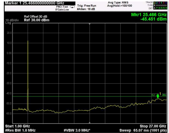
Channel: TOP, Modulation: 256QAM, BW=10MHz, Range: 1GHz - 27GHz
