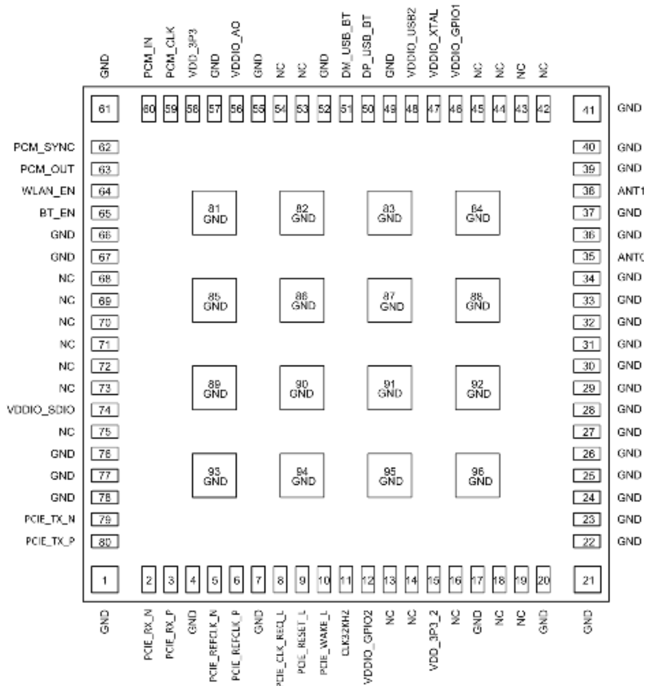
Figure 2: BALI PCIe Pin Diagram
