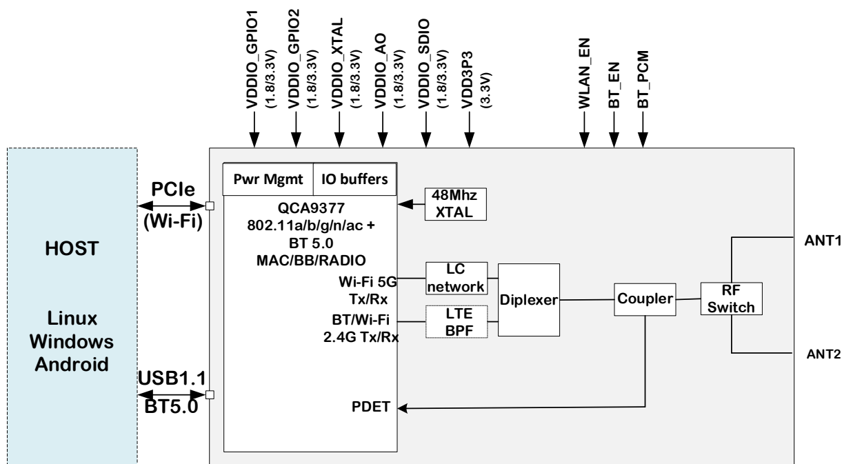
Figure 1: BALI PCIe Block Diagram with Antenna Pin
