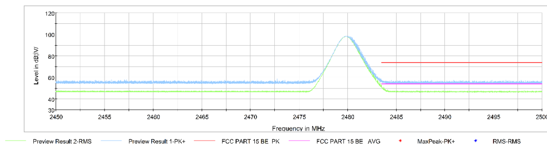
Fig.14. Frequency Band Edges: GFSK, Channel 78, Hopping Off, ch11, 2.45 GHz - 2.50GHz
