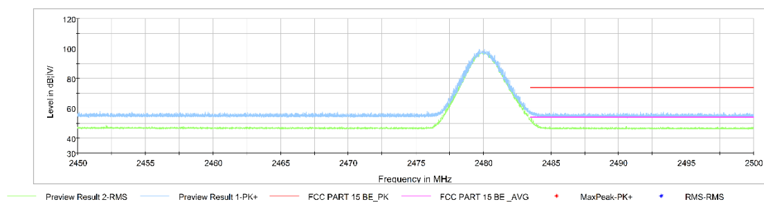
Fig.18. Frequency Band Edges: 8DPSK, Channel 78, 2.45 GHz - 2.50GHz
