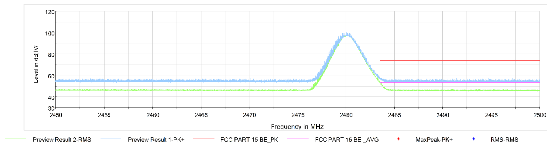
Fig.16. Frequency Band Edges: \pi/4 DQPSK, Channel 78, Hopping Off, 2.45 GHz - 2.50GHz
