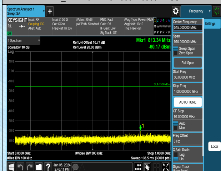
BLE_1M-Ant2-2440-30~1000-PASS
